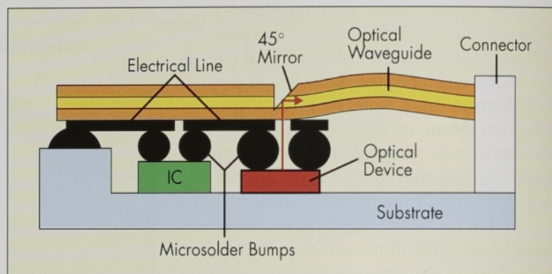
Schematic representation of optoelectronic chip-on-film packaging.
