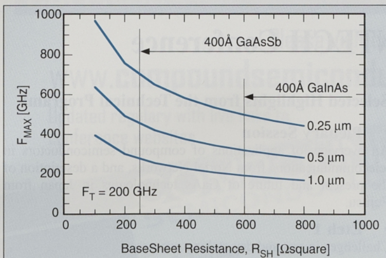
Figure 5. f_{MAX} dependence on the base sheet resistance for various design rules in conventional mesa DHBTs for f_T = 200 GHz. The very low RSH achievable in heavily doped GaAsSb:C is expected to yield record f_{MAX} values for mesa transistors. Much lower sheet resistances are achievable with GaAsSb than with GaInAs.
