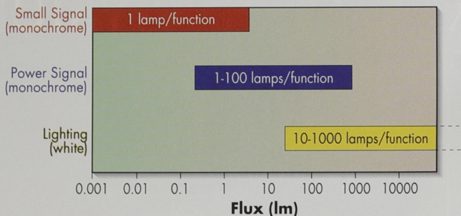
Figure 3. A classification scheme for the major categories of LED applications, based on the required output (in lumens) and the number of die required.
