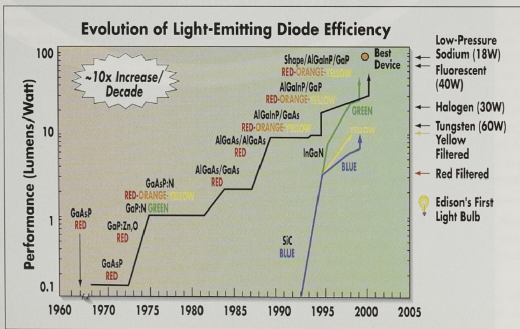
Figure 1. Chart illustrating “Craford’s Law”.
