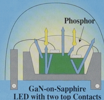
GaN + Phosphor LED
