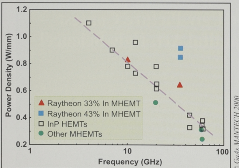
Figure 1. Comparison of recently published power density results for metamorphic GaAs HEMTs and InP HEMTs (for devices with >150 \mu\text{m} periphery). Courtesy of Colin Whelan, Raytheon RF Components.
