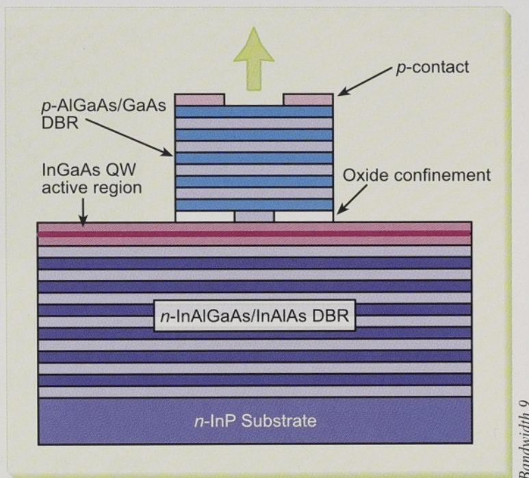
Figure 1. Schematic showing the structure of Bandwidth9's single-epitaxy, top-emitting 1.6 \mu m VCSEL.
