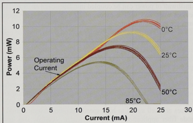
Figure 4. Gore's VCSEL arrays are designed to have very stable performance over temperature at the actual operating current of \sim 5 mA. This simplifies the system design, and eliminates the need for a monitor photodiode feedback loop.
