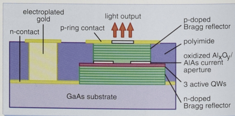
Figure 1. Schematic layout of a low-parasitic, top-emitting VCSEL.
