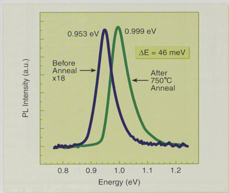
Figure 1. PL spectra of an \text{In}_{0.35}\text{Ga}_{0.65}\text{As}_{0.982}\text{N}_{0.018} MQW structure before (left) and after (right) annealing at 750°C.
