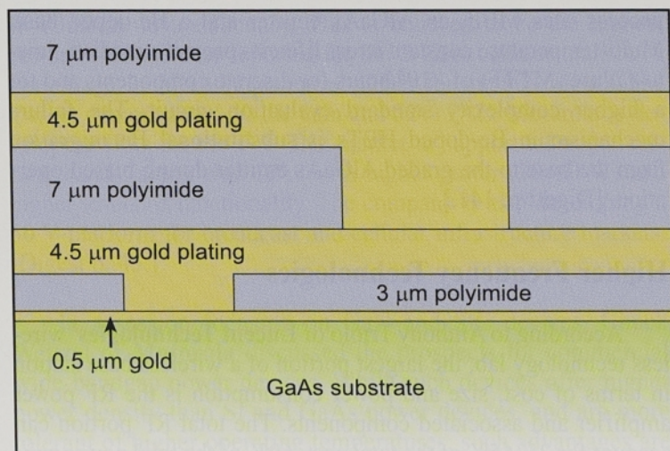
Figure 4. The multi-level plating (MLP) process adds a second layer of thick gold plating and a second layer of polyimide interlayer dielectric to M/A-COM's existing process for fabricating RFICs and MMICs. Courtesy of John Dille, M/A-COM.
