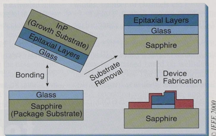
Schematic illustration of NTT's integrated packaging technology.
