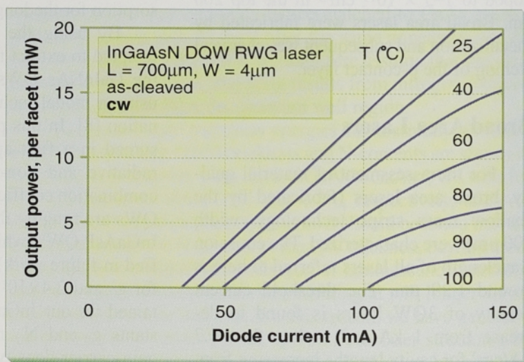
Figure 4. High temperature CW operation of a 700- \mu\text{m} -long, as-cleaved ridge waveguide laser emitting at 1.30 \mu\text{m} . T_0 is measured to be 110 K.
