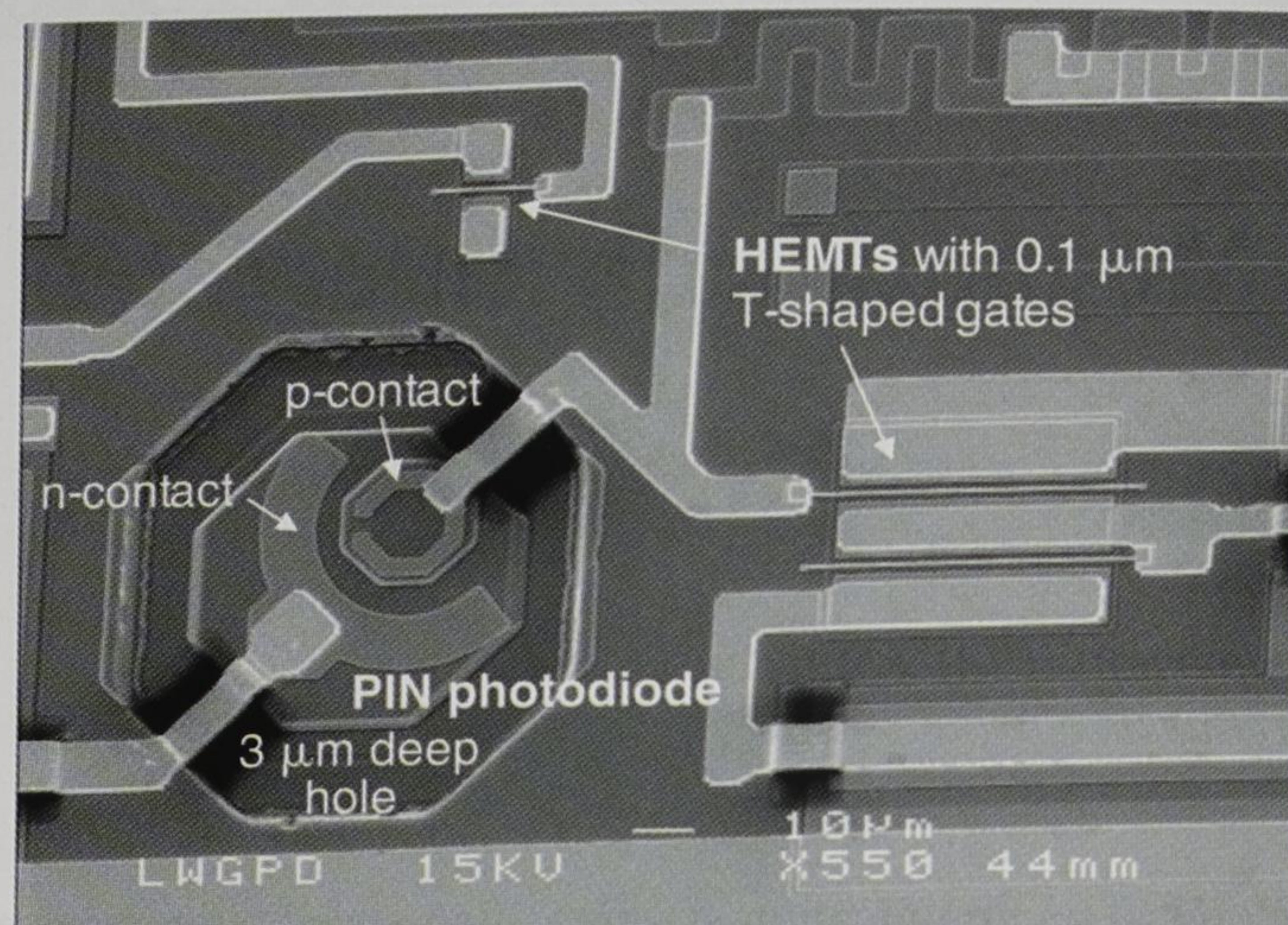
Figure 3. SEM micrograph of a part of a PIN-HEMT circuit. The photodiodes have a diameter of 23 \mu m.
