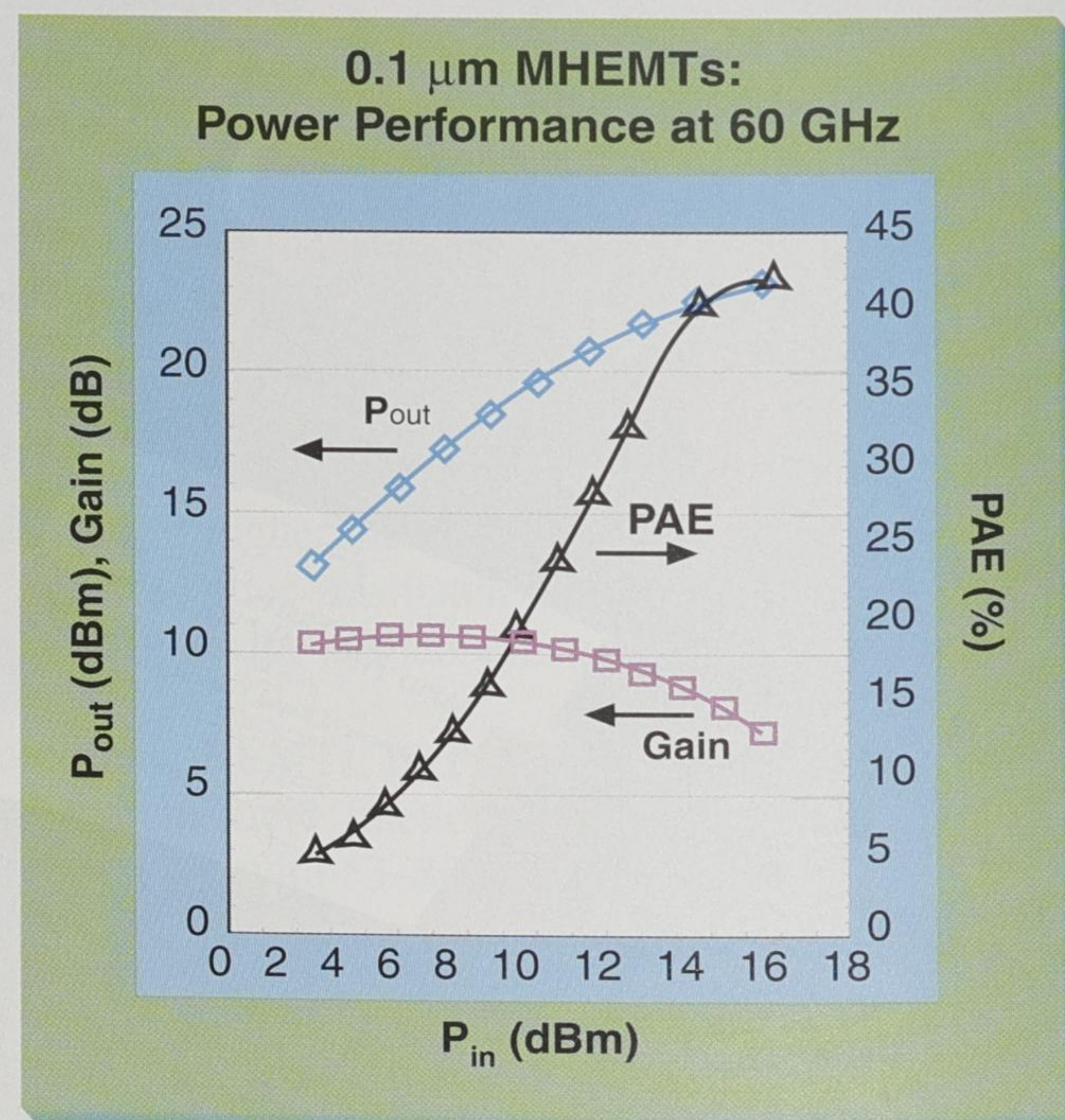
Figure 5. Power performance of 0.1 \mu\text{m} MHEMT MMICs.
