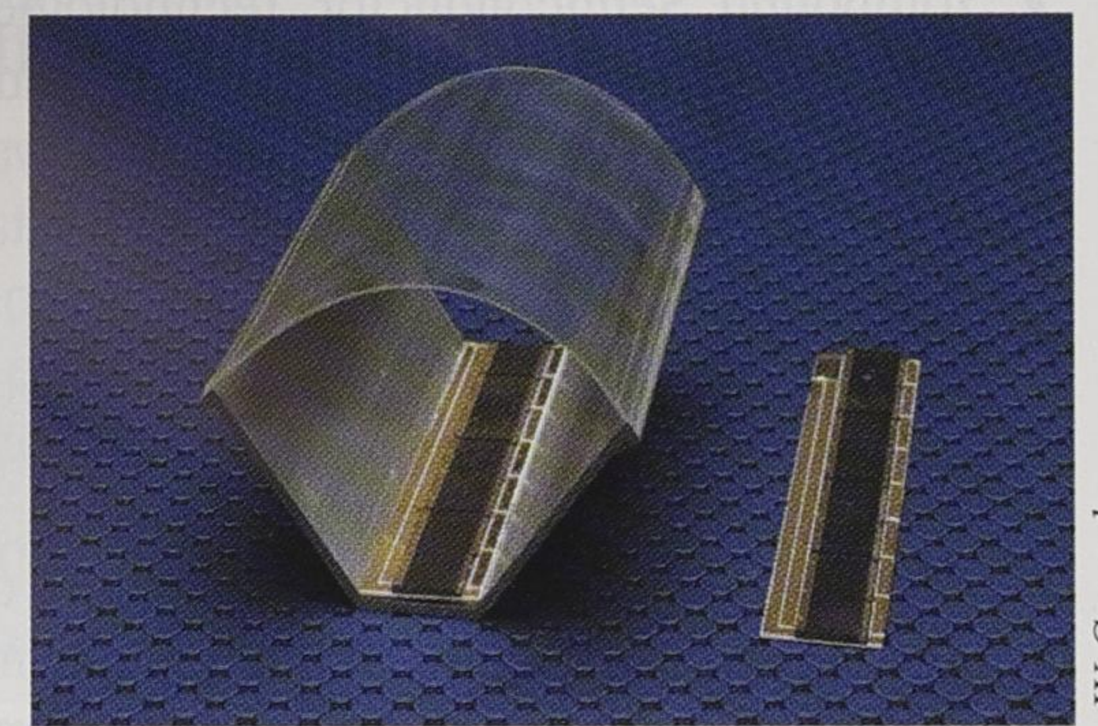
Figure 2. The Tecstar/ JX Crystal module contains cell-interconnected-circuit (CIC) assemblies consisting of two GaInP/GaAs dual junction front cells stacked with seven GaSb boosters cells. An arched Fresnel lens solar concentrator supplied by Entech focuses solar radiation onto the detector, and may result in efficiencies as high as 35% at 15 suns AM0.
