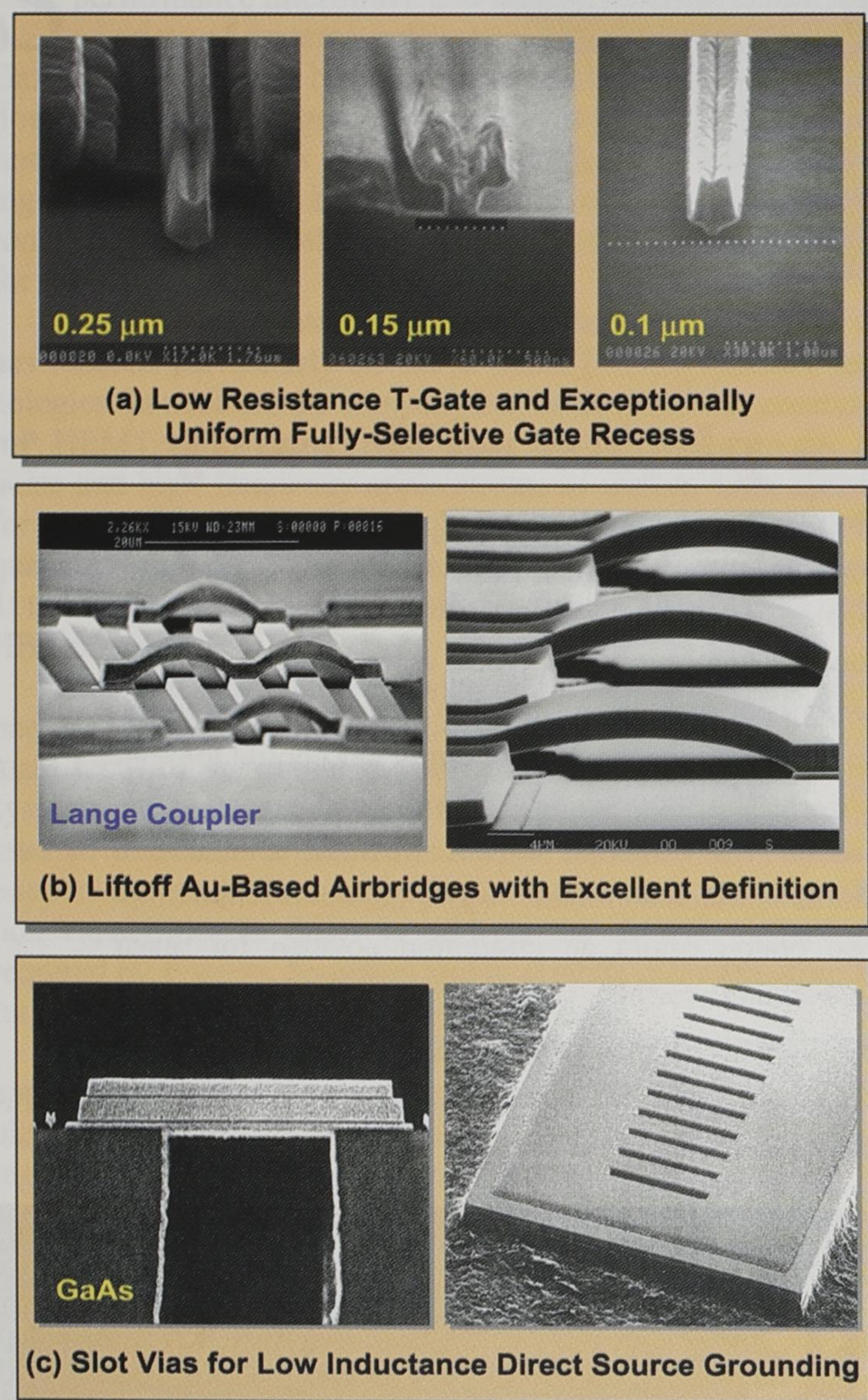
Figure 3. Highlights of Sanders' metamorphic HEMT technology.
