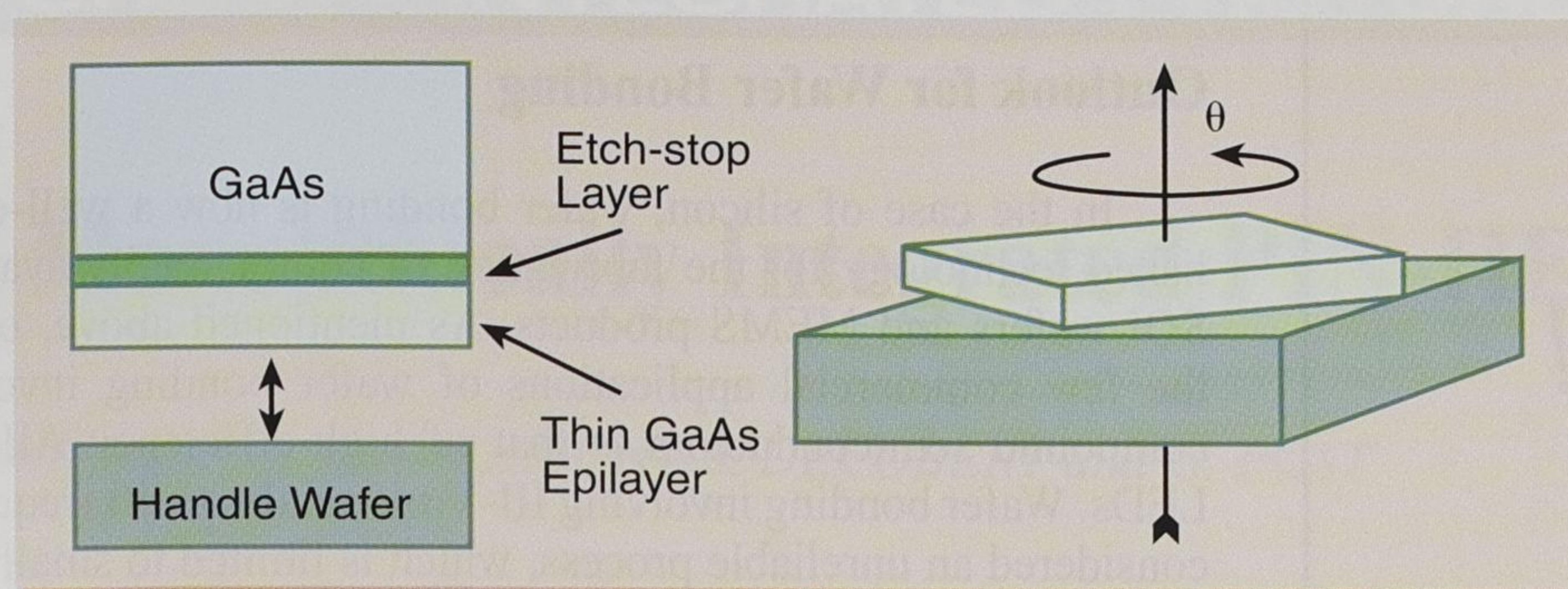
Figure 6. Schematic of twist-wafer bonding used for fabrication of compliant substrates.
