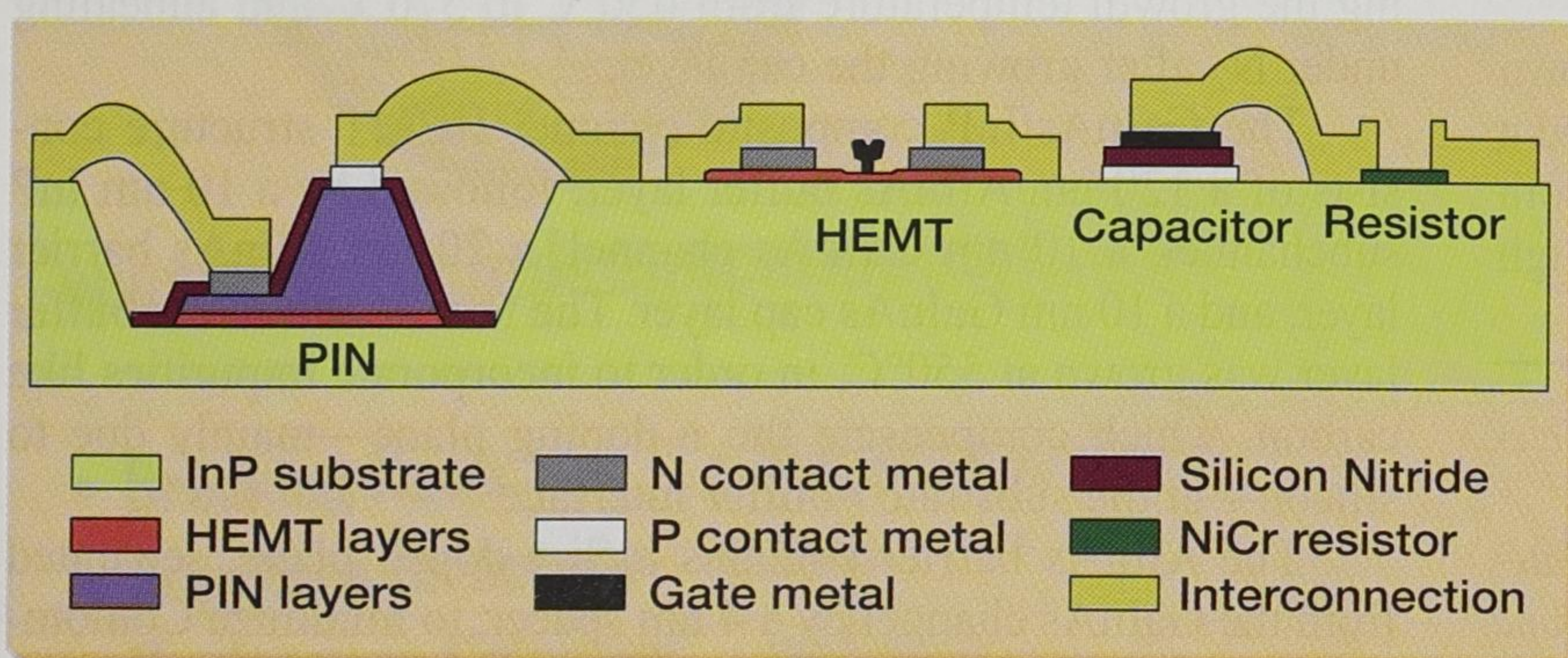
Figure 2. Cross-section of the PIN-HEMT OEICs after processing.
