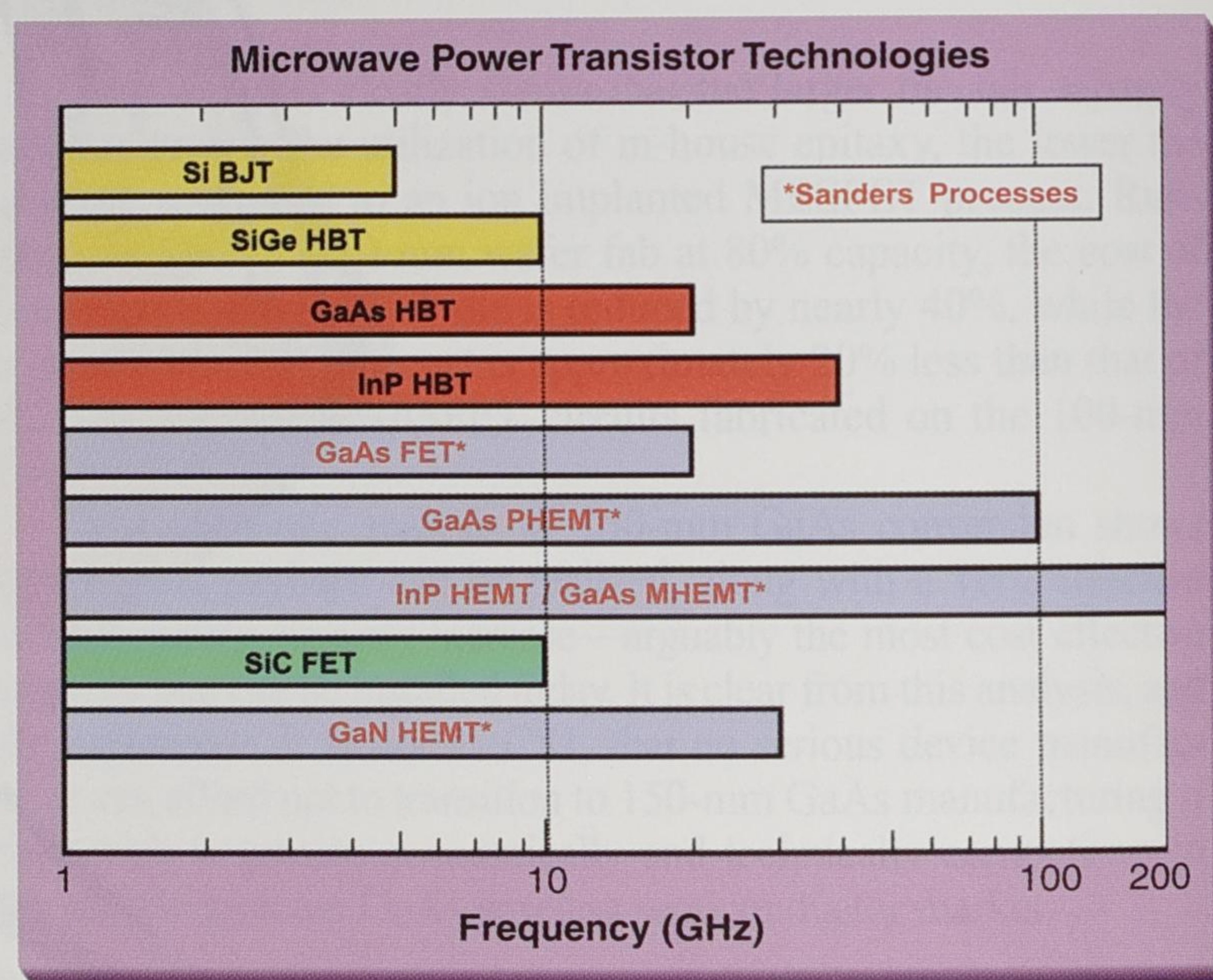
Figure 1. Applicable frequency range for microwave power technologies.
