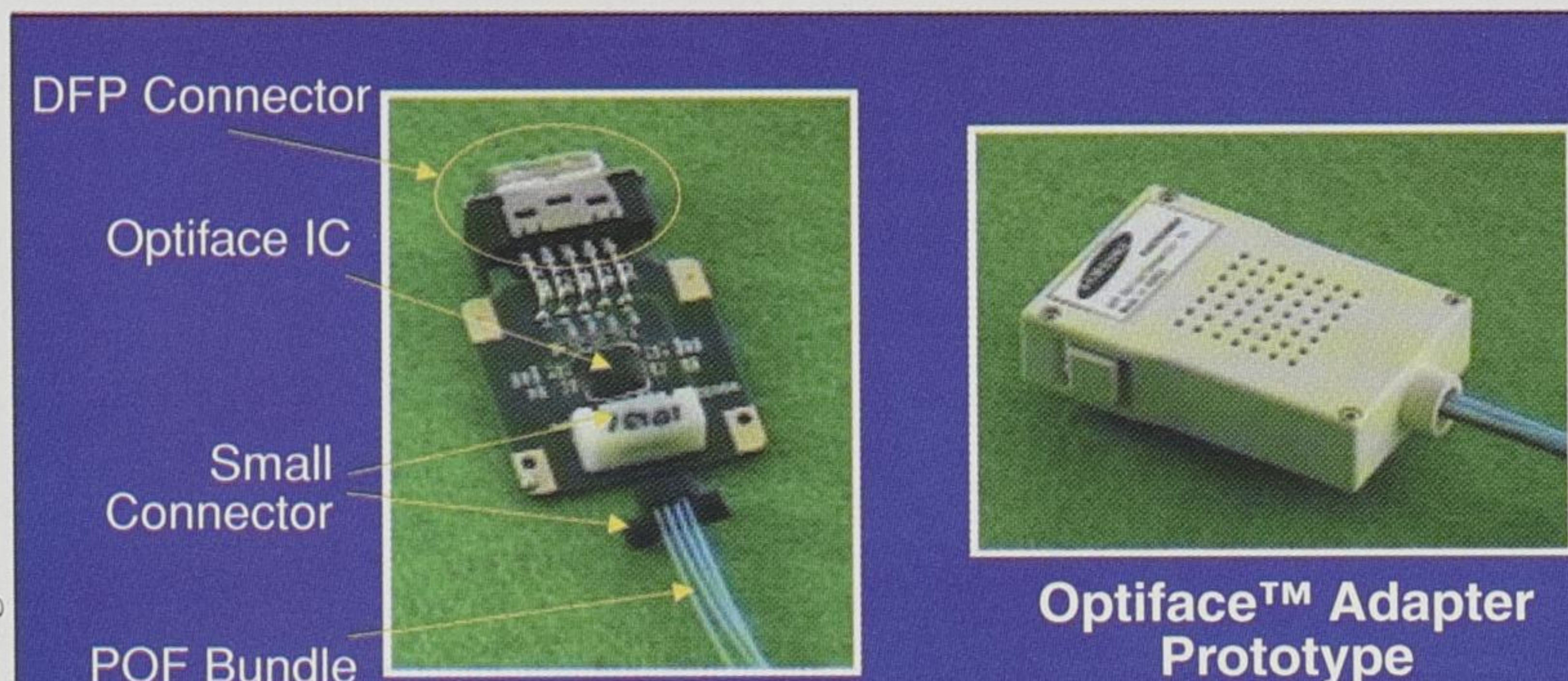
Figure 4. A prototype Optiface™ adapter that converts electrical signals from the DFP connector into optical signals for transmission through the plastic fiber bundle.
