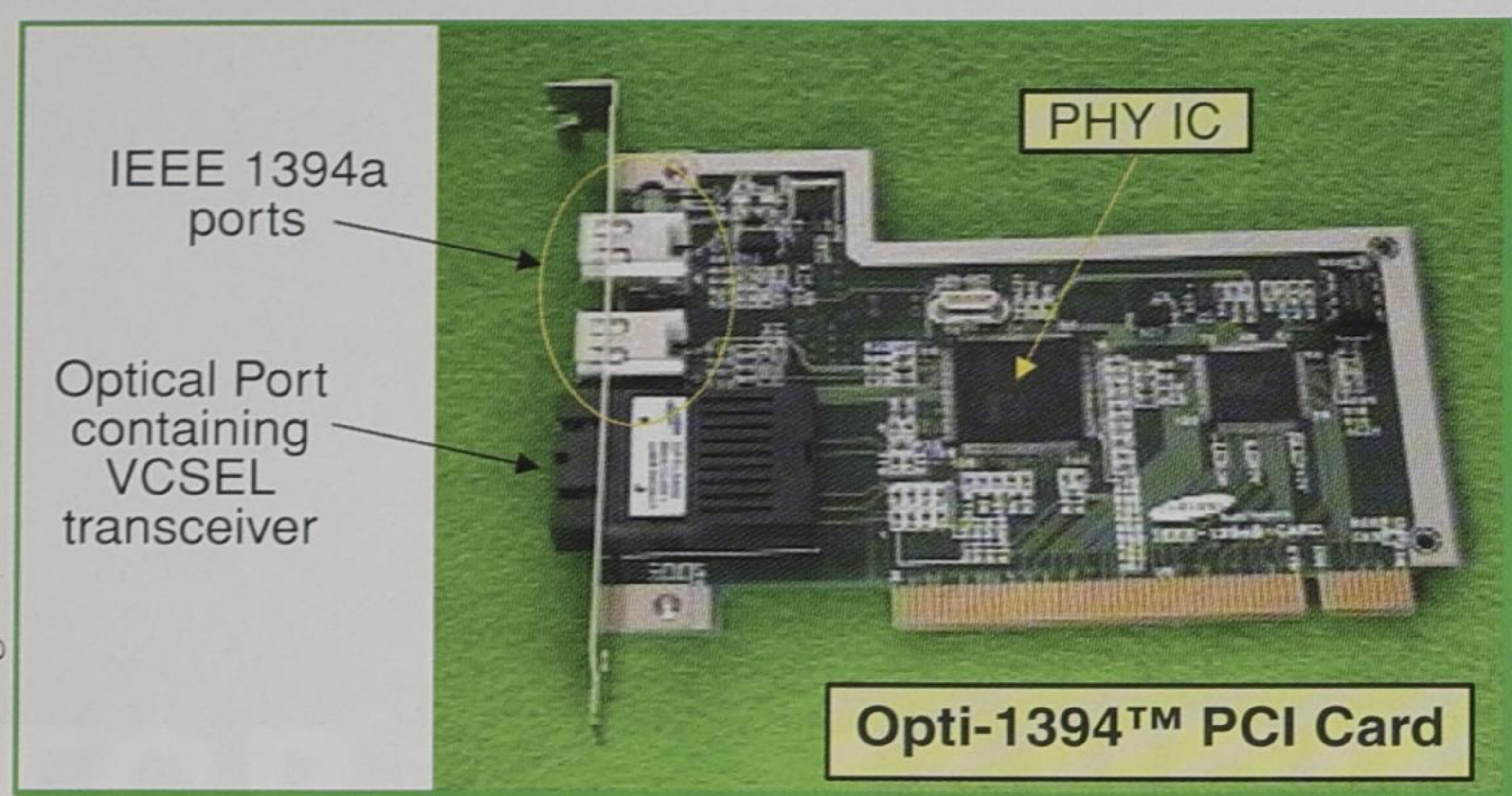
Figure 2. Samsung has demonstrated PCI cards that are suitable for providing optical connections directly to a PC.
