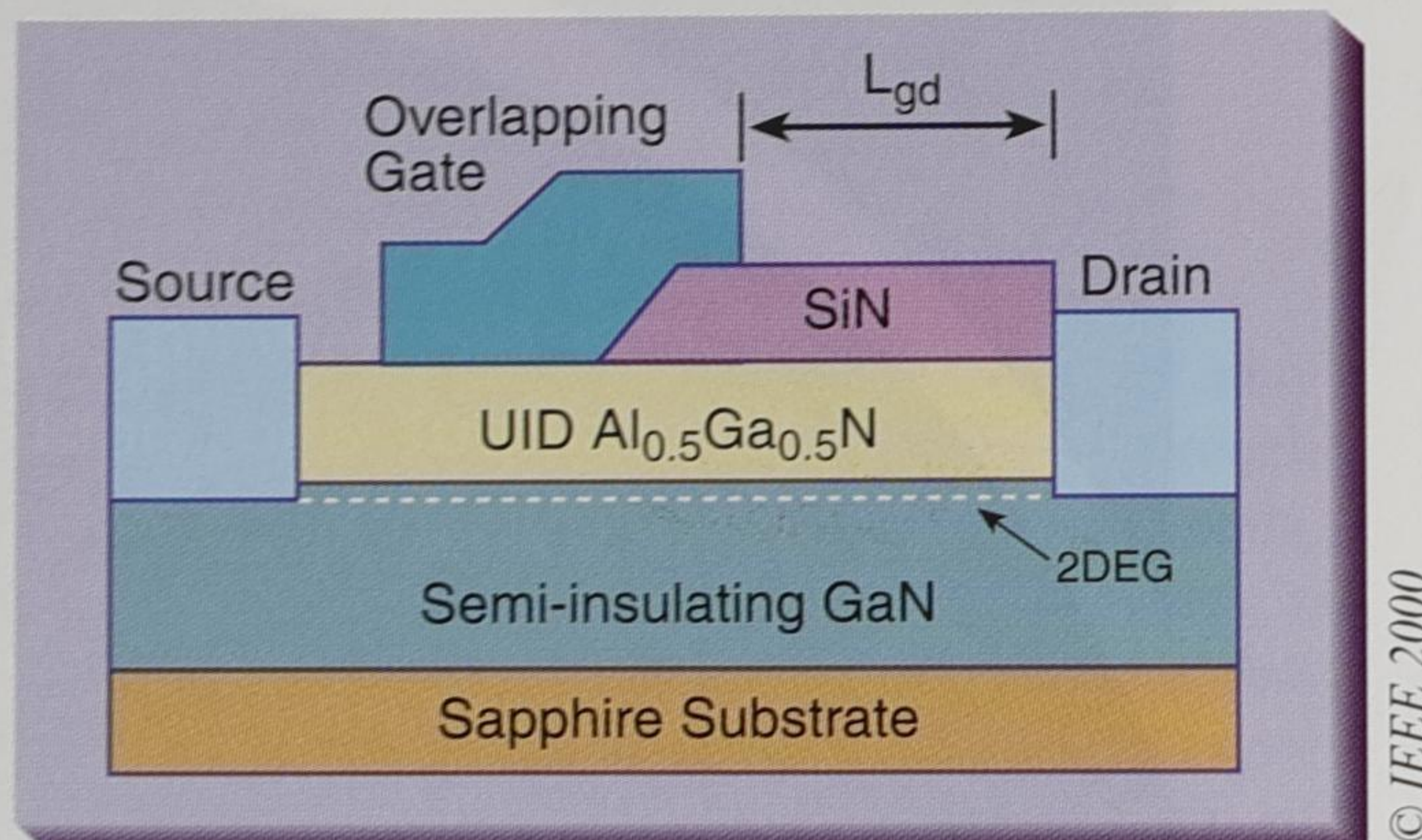
Schematic diagram of a AlGaIn/GaN HEMT with an overlapping gate structure.
