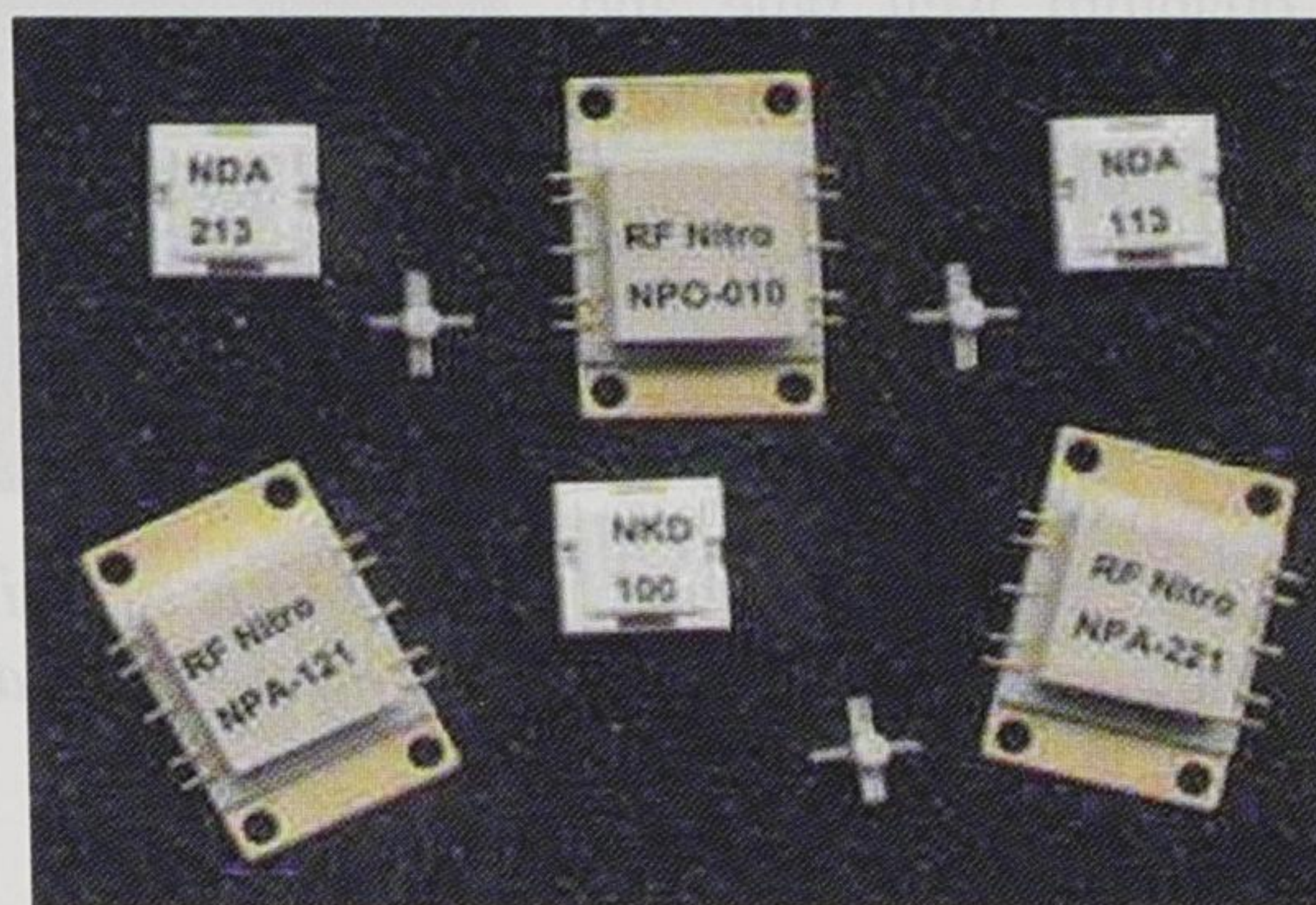
Figure 2. Surface mount GaAs devices for use in high power PAs, frequency doublers and VCOs operating in the microwave and millimeter wave band.
