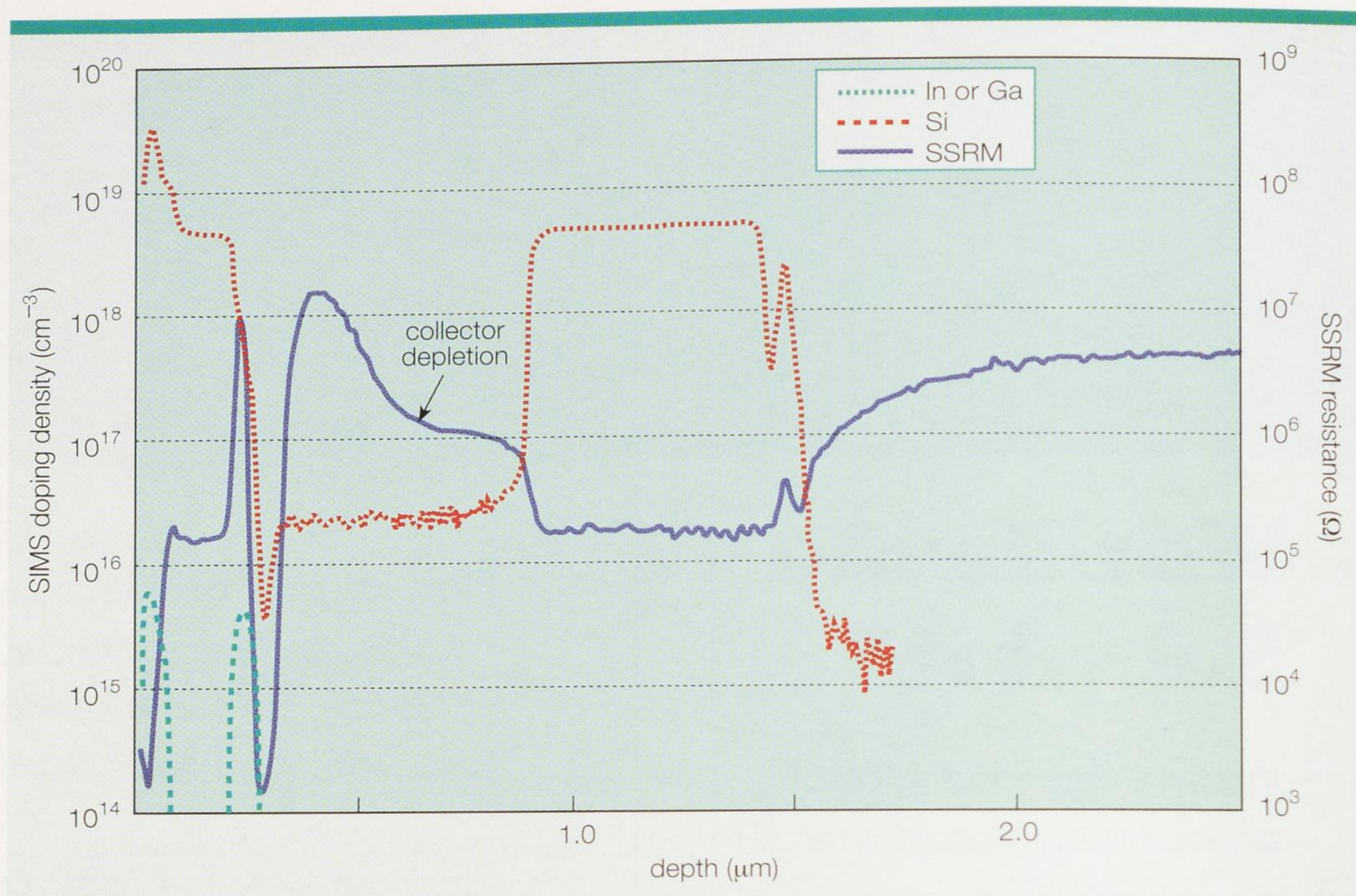
Fig. 4. A comparison of the SIMS and SSRM profiles of a GaInP/GaAs HBT structure. The SSRM scale on the right (resistance) accurately correlates with the doping density as measured by SIMS. In this structure a depletion region is evident in the collector.
