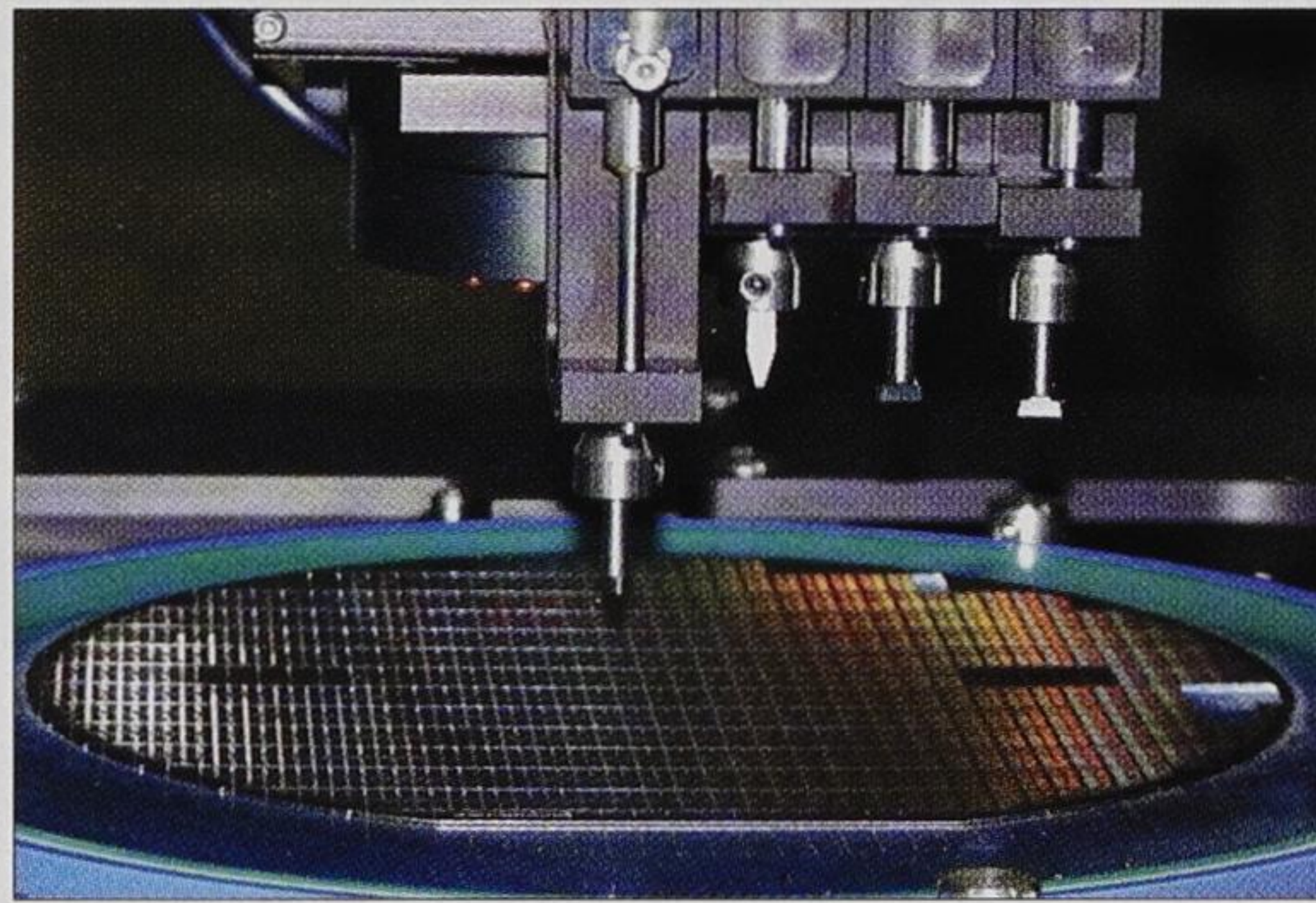
MRSI manufactures component assembly dispensers and automated assembly and packaging systems, including this eutectic die-attach-from-wafer unit.
