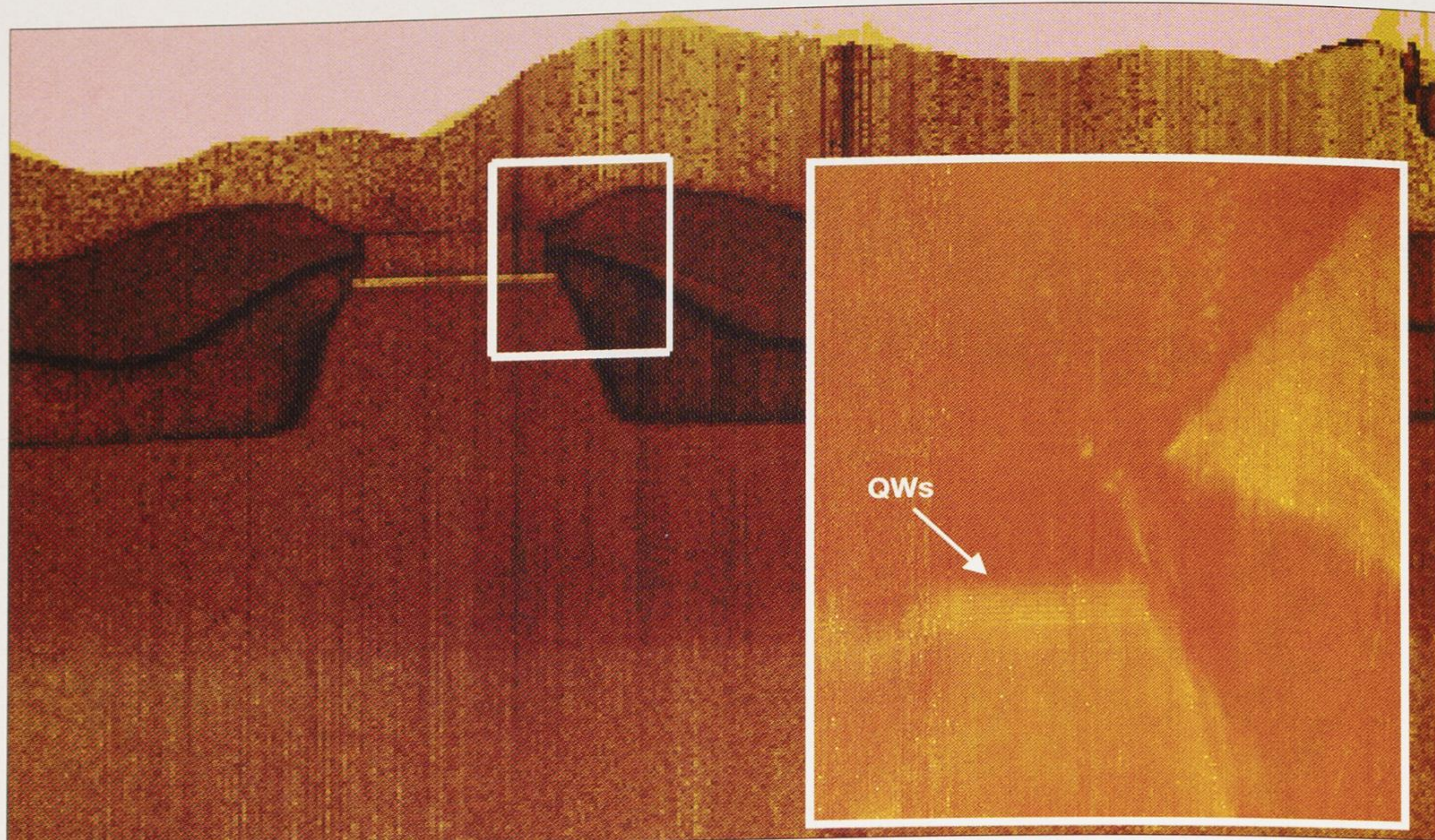
Fig. 3. Cross-section SSRM image and (inset) expanded view of the active area in an InP buried heterostructure laser. The lateral extent of the main image is 10 \mu\text{m} and the inset resolves the \sim 5 nm quantum wells (QWs).
