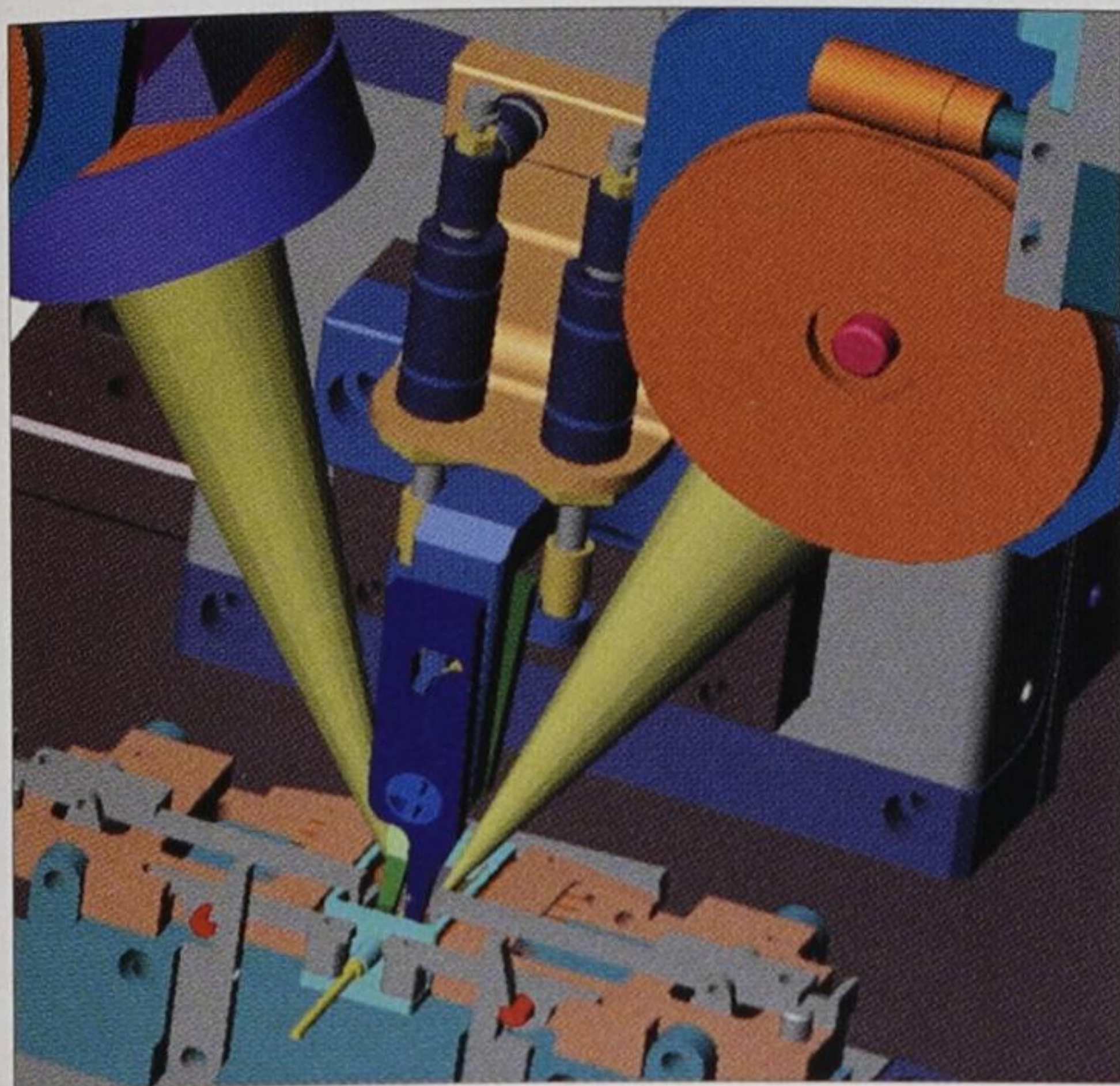
Fig. 4. Collision detection analysis can be carried out by 3D simulation.
