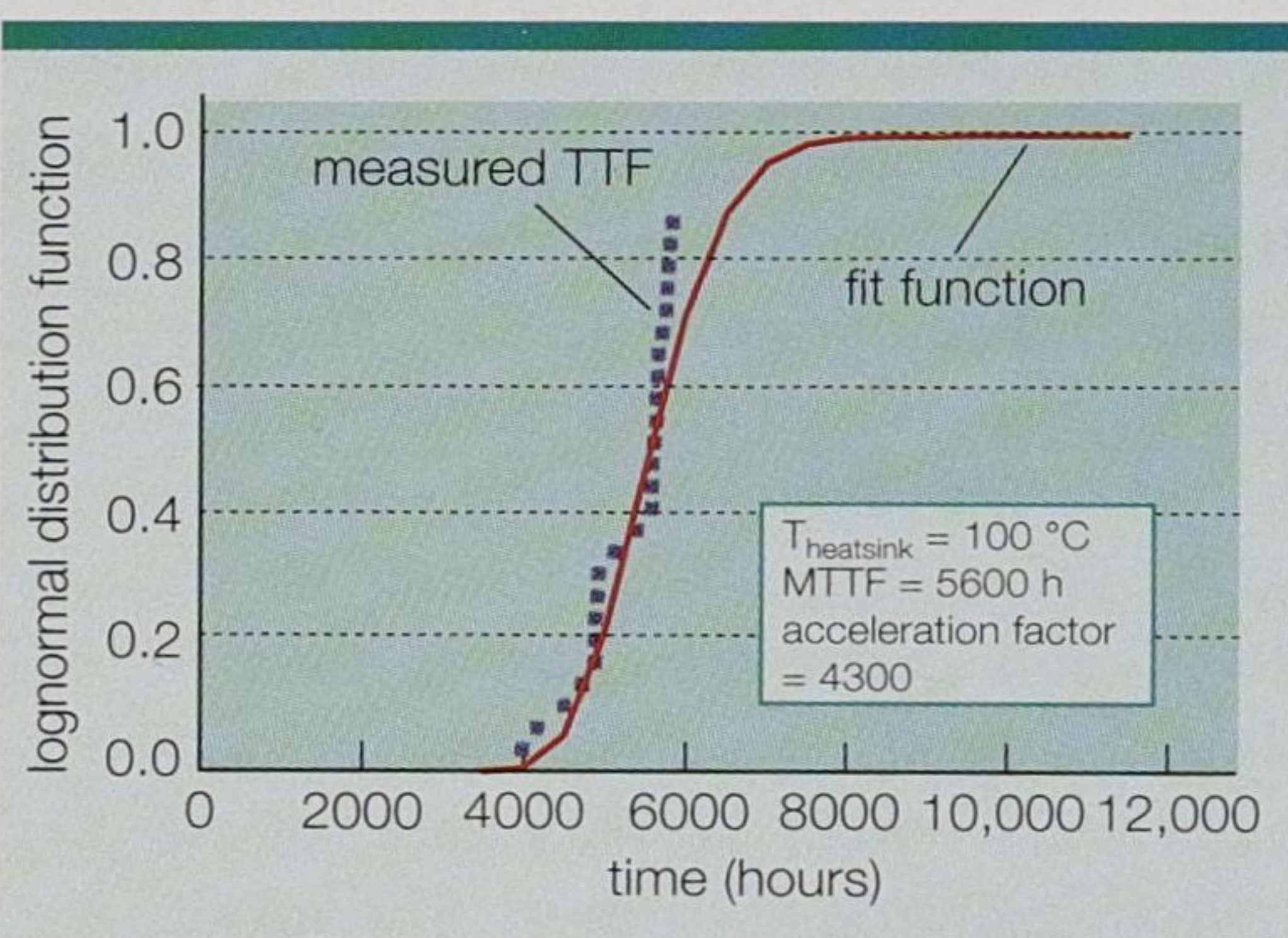
Fig. 5. Log normal plot versus time-to-failure (TTF), which is used to determine mean-time-to-failure (MTTF) values.
