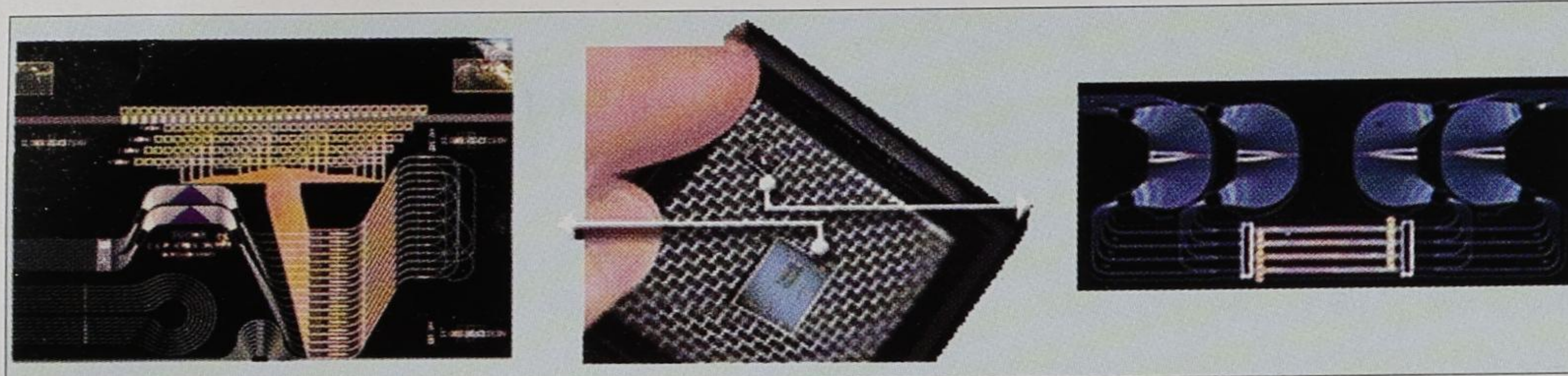
Fig. 2. The chip on the left measures 12 mm × 9 mm and demonstrates the complexity of optical waveguide structures that can be fabricated in InP. The chip on the right is a four-wavelength 2 × 2 optical cross-connect measuring 1.5 mm × 3.3 mm 2 . This device is fabricated from InP and is the smallest ever produced.
