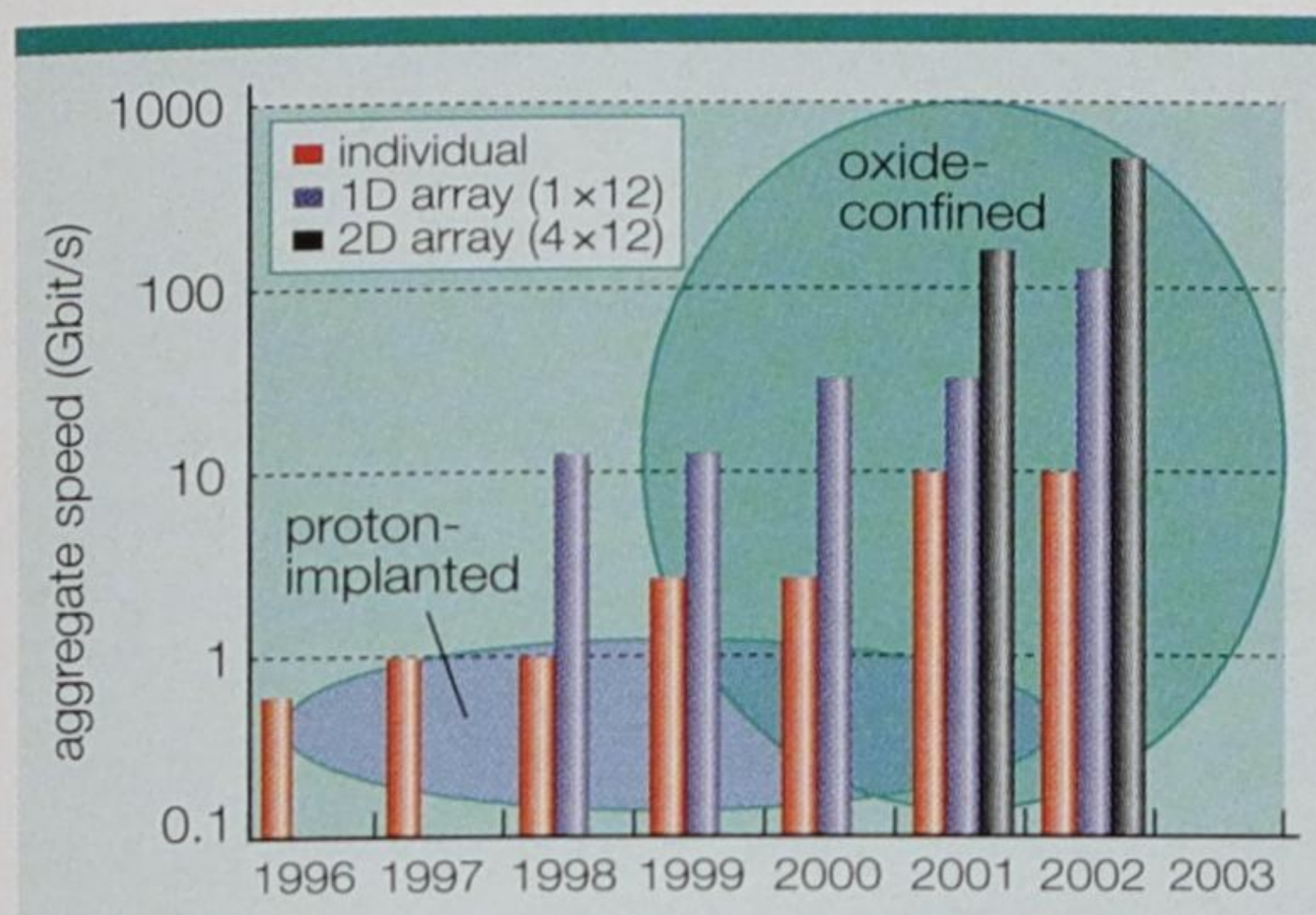
Fig. 1. Since the first appearance of VCSELs, the aggregate bandwidth has been increased due to the higher modulation speeds of individual lasers, and the fabrication of 1D and 2D arrays.
