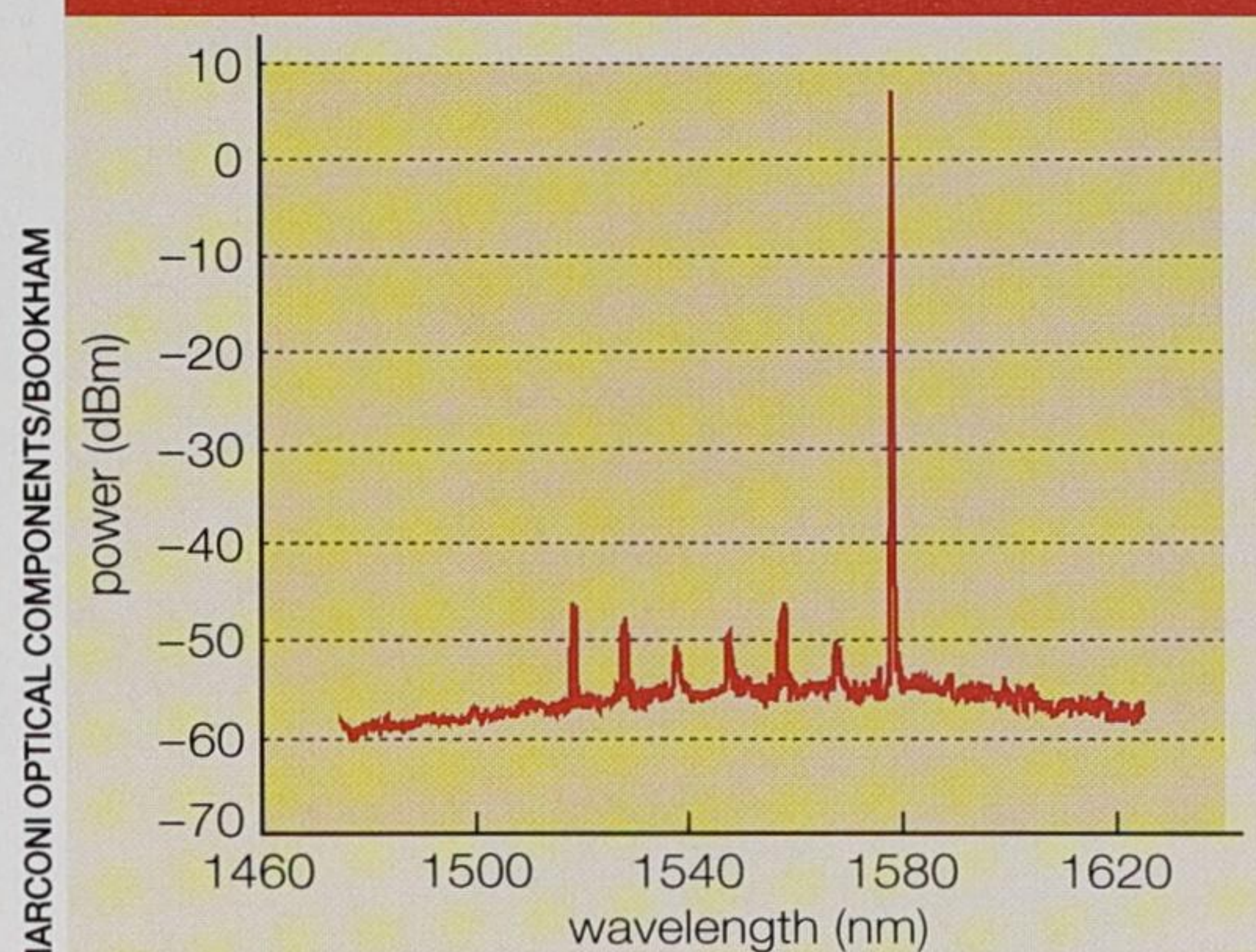
Spectra of peaks from one supermode of the DS-DBR laser. Fine-tuning allows the selection of a single peak with greater than 50 dB sidemode suppression.
