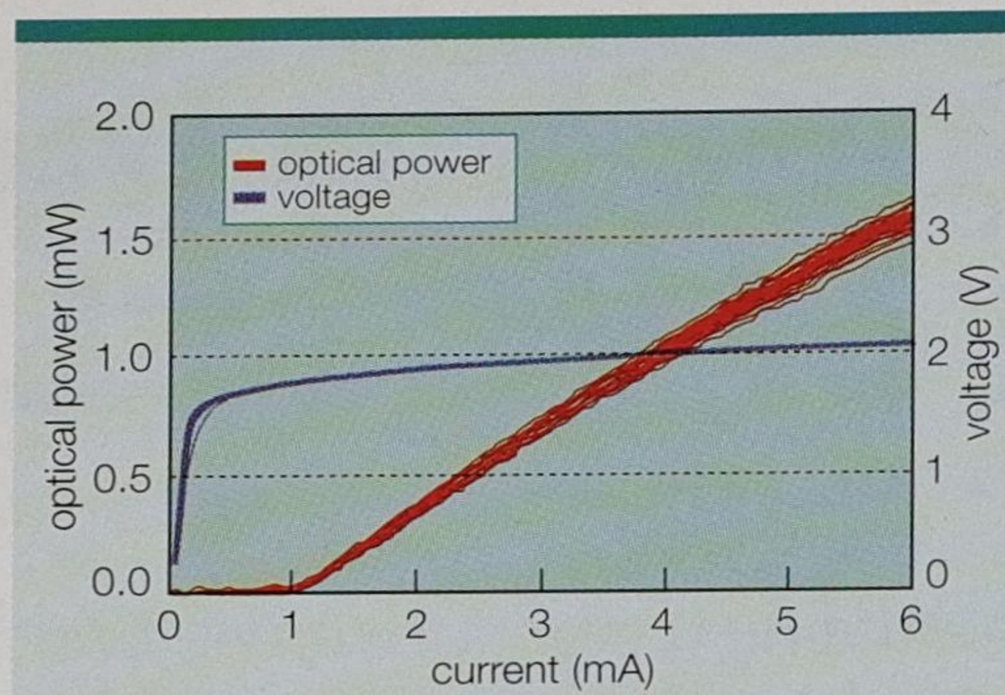
Fig. 3. The LOI characteristics of a 4 \times 12 bottom-emitting VCSEL array flip-chip that has been mounted on a subcarrier after substrate removal. The active diameters are 10\text{ }\mu\text{m} and measurements are taken at room temperature.
