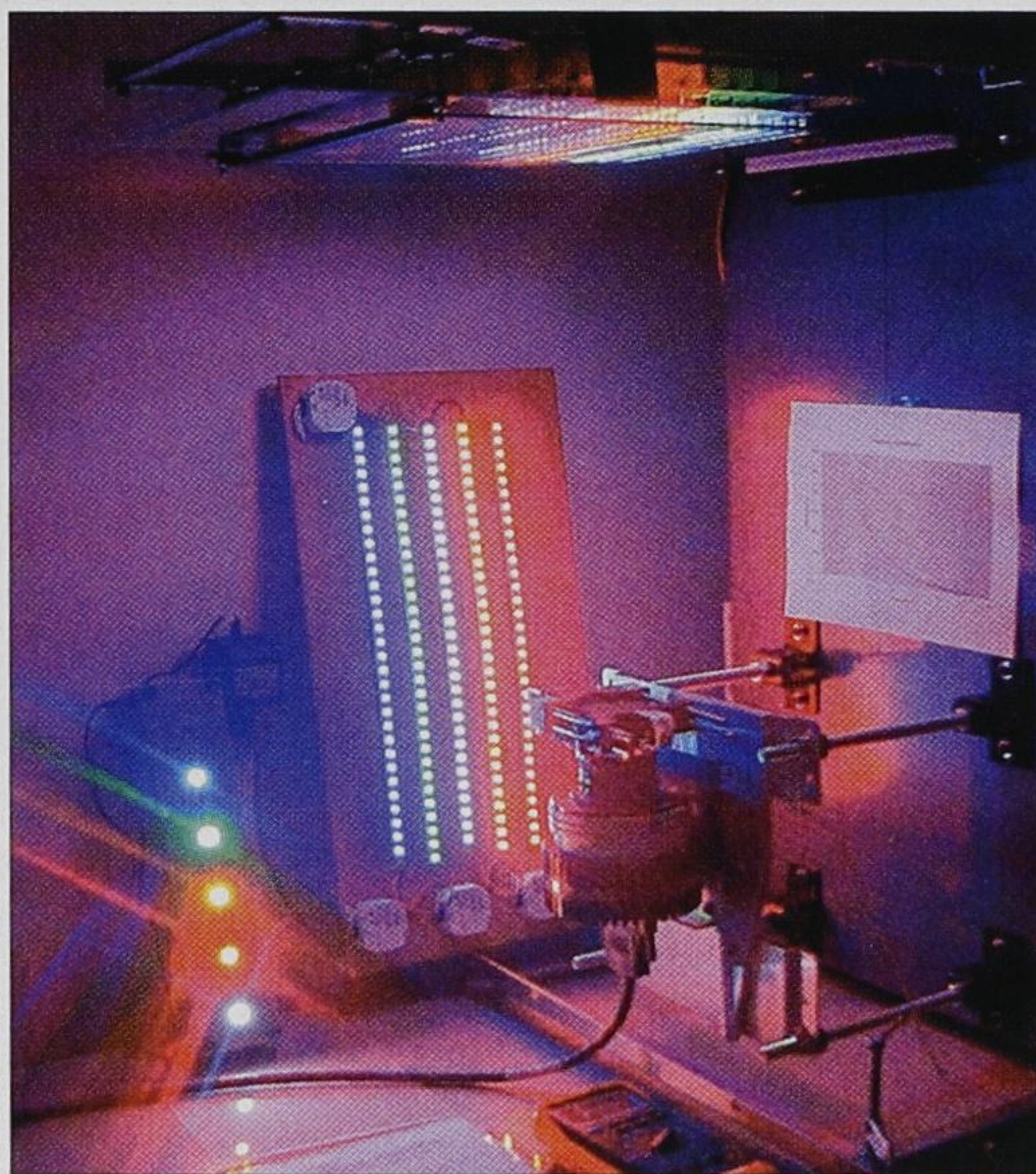
LEDs undergoing lifetime testing at the Lighting Research Center.
