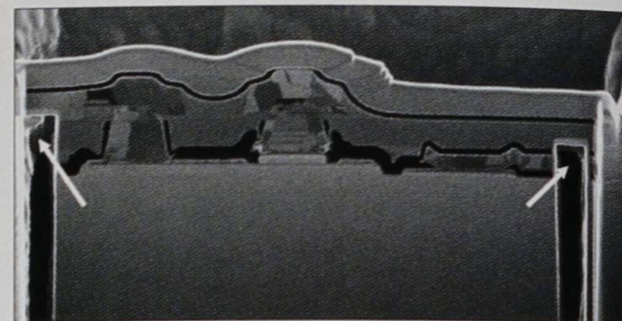
Fig. 5. SEM image of a completed TEM lift-out sample obtained from an HBT, thinned using FIB. The resulting foil contains slots (indicated by arrows) where the specimen is snapped off for imaging in the TEM.
