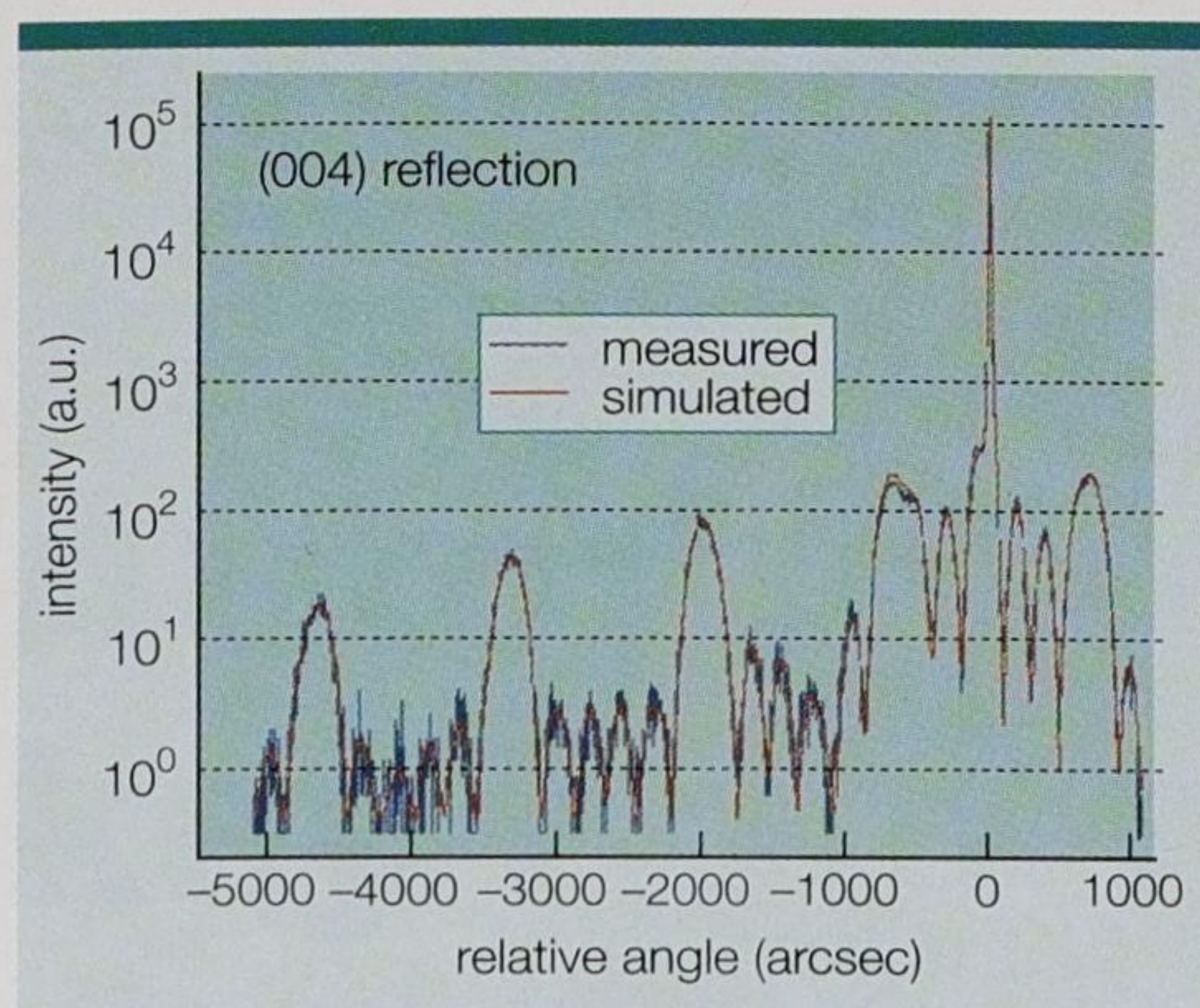
Fig. 7. High-resolution computer simulations of rocking curves obtained for an InAlAs MQW laser structure. The large peaks arise from the MQW period, while the higher frequency peaks are generated by the bulk InP layers.
