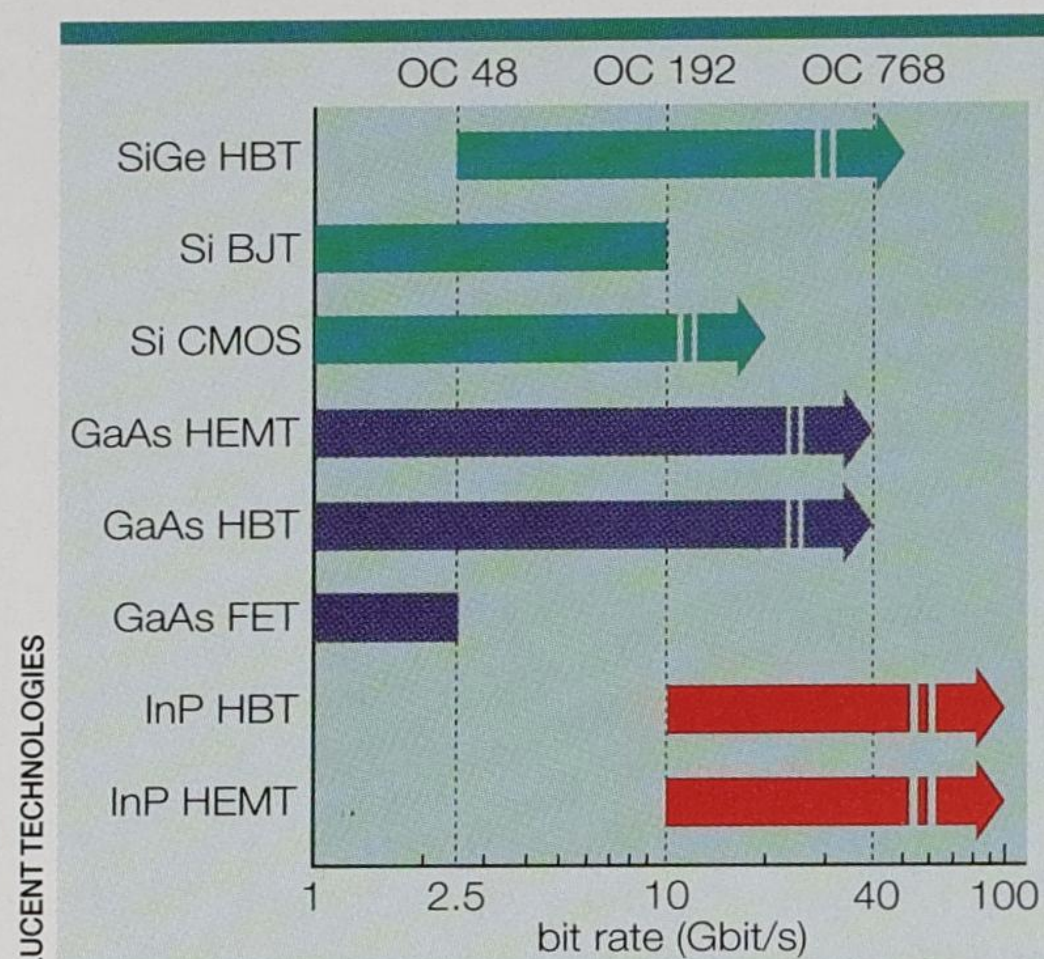
Fig. 3. As silicon ICs approach maximum operating speed, InP electronics could be a full order of magnitude faster. Since it can also outperform GaAs, InP is the preferred platform for monolithic integration.
