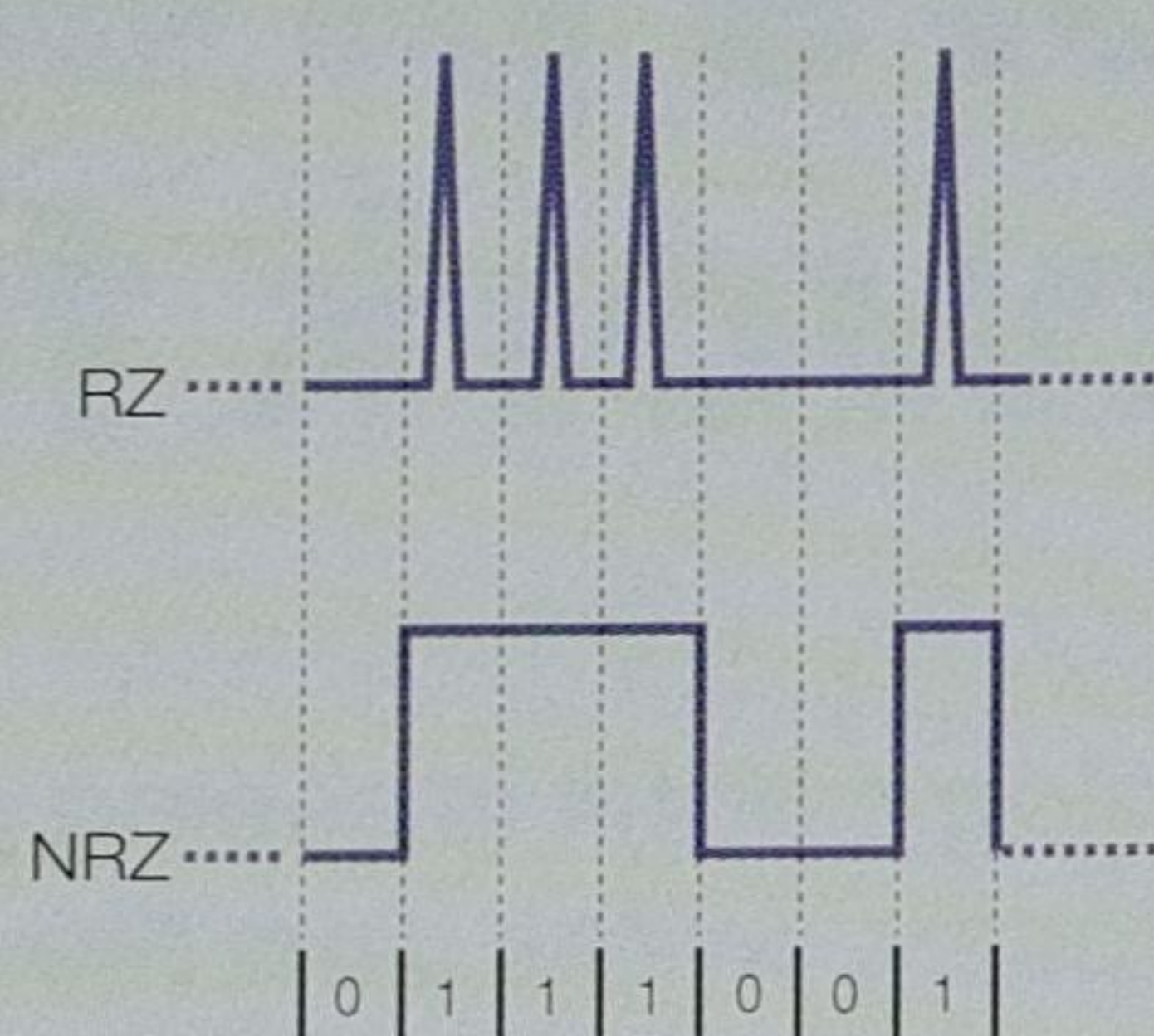
Fig. 1. In RZ modulation a light pulse represents a 1 in the data stream. The light returns to 0 after each 1, even if there are consecutive 1s. In NRZ modulation the light stays on until a 0 is encountered.
