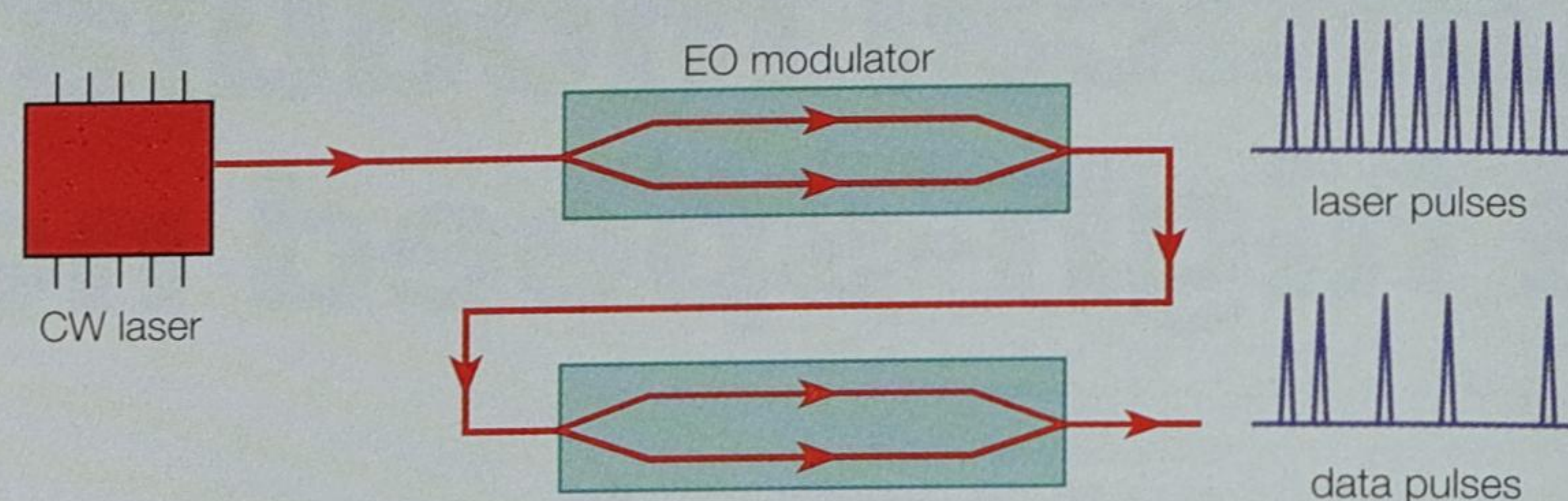
Fig. 2. Two modulators are required for RZ modulation. The first generates a stream of pulses from a CW laser. The second modulates these pulses to generate the data stream.
