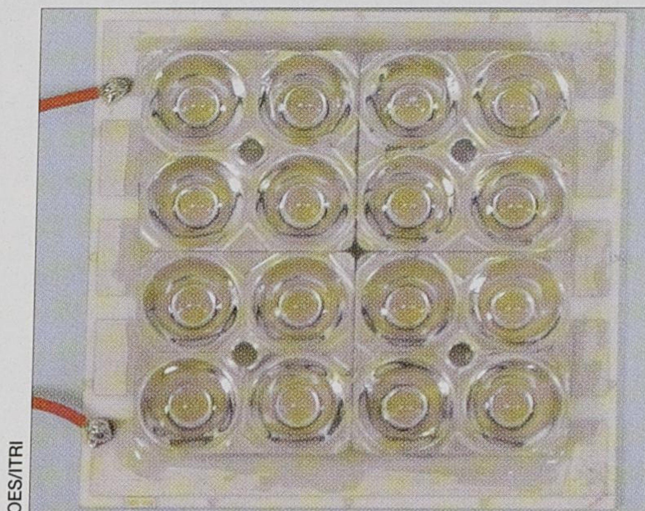
An LED module containing a total of 64 LED chips, which are surface-mounted to a board (measuring 5 × 5 cm 2 ) and coated to form focusing lenses.
