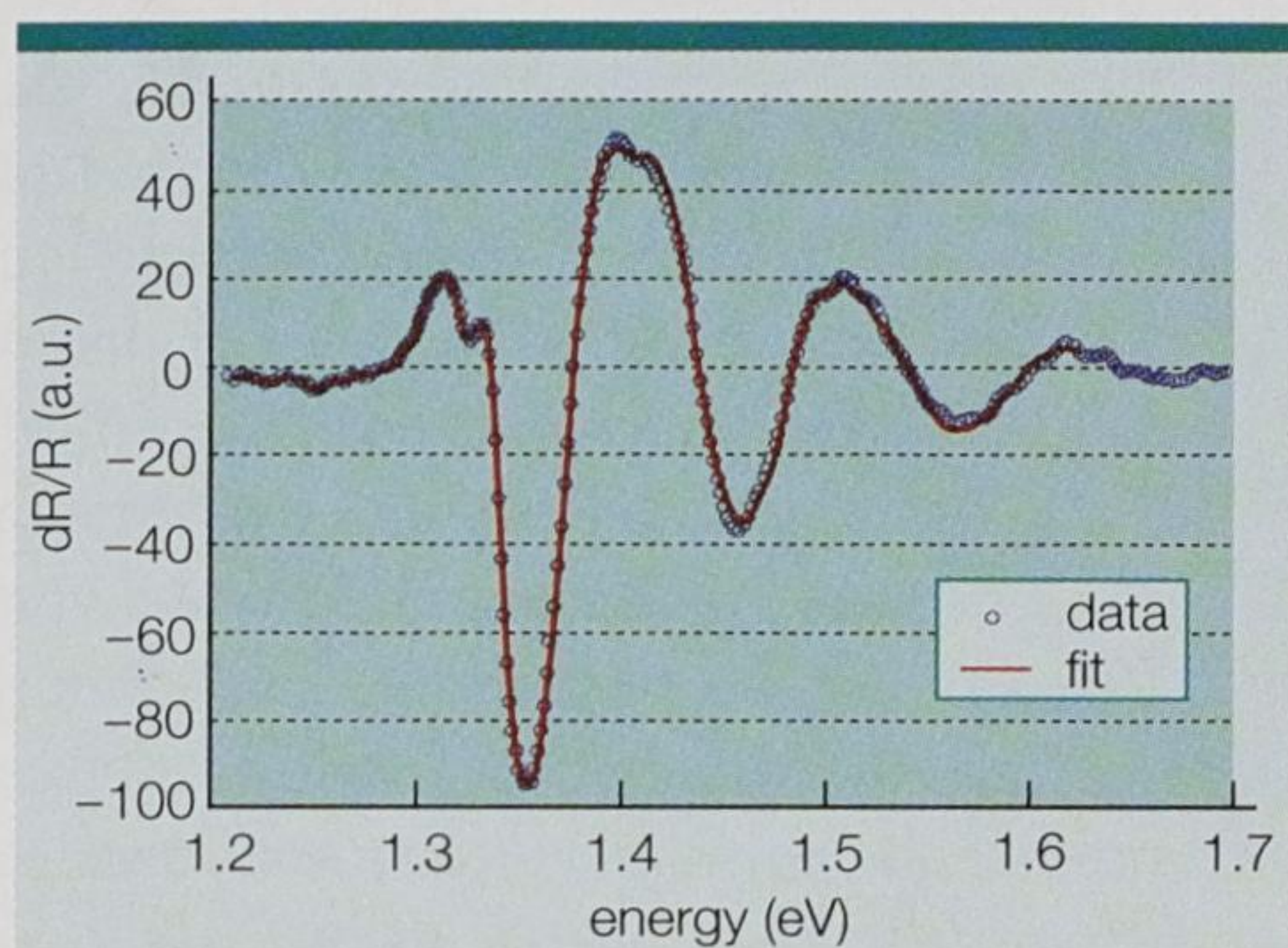
Fig. 8. Simulation of a photoreflectance modulation spectrum taken from an InP double heterostructure HBT. The simulation deconvolves the spectrum of the more heavily doped emitter (higher bandgap and field) from the lightly doped collector.
