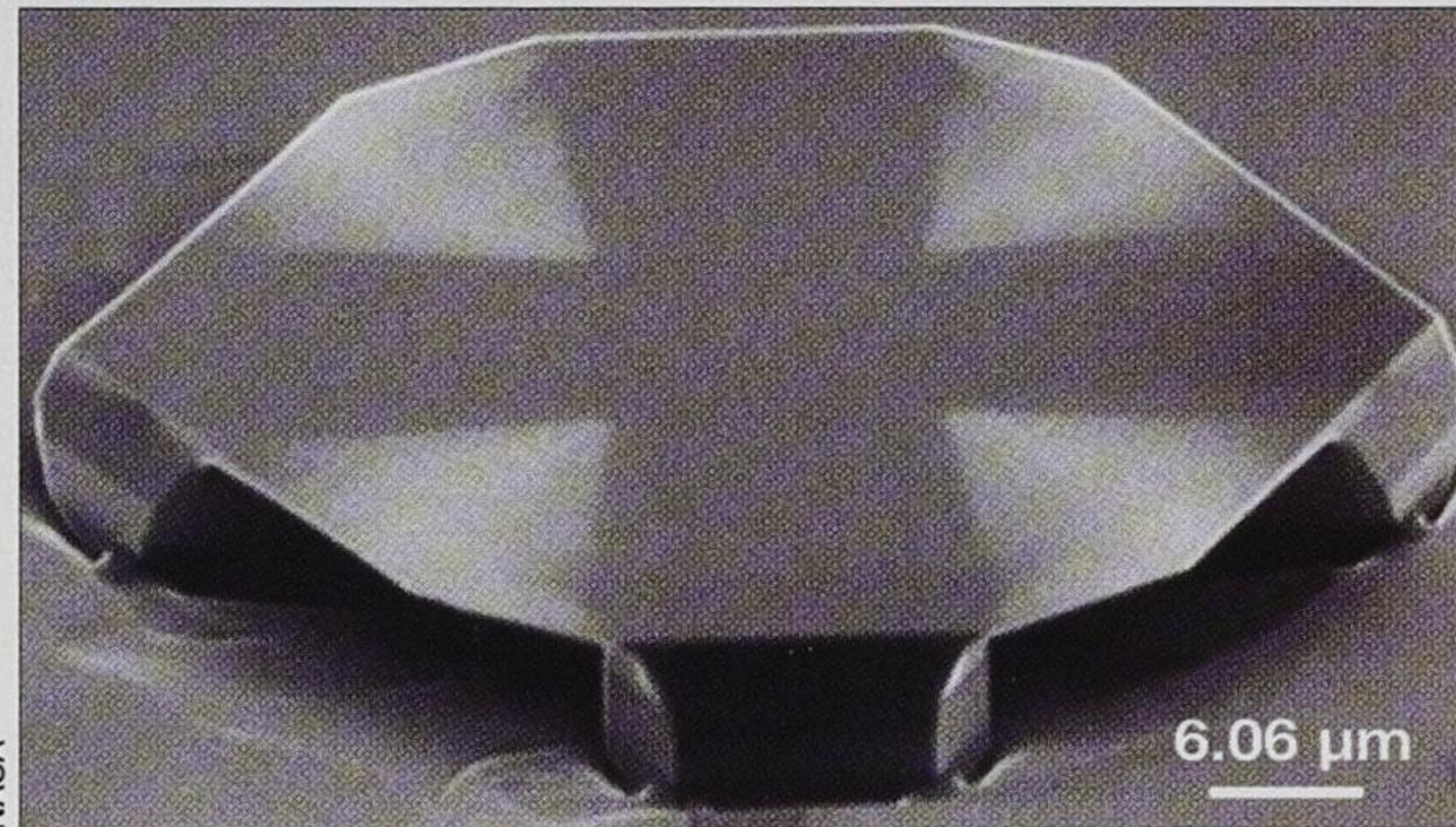
A step-free 4H-SiC surface grown using web growth. The original mesa is visible as the dark cross. The lighter V-shaped areas are the web-grown material.
