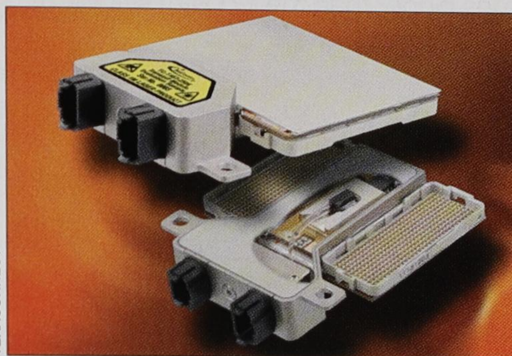
TeraConnect's modules contain arrays of VCSELs or detectors aligned with ferrules that feed into polymer waveguides, which are visible in the foreground of the cutaway.
