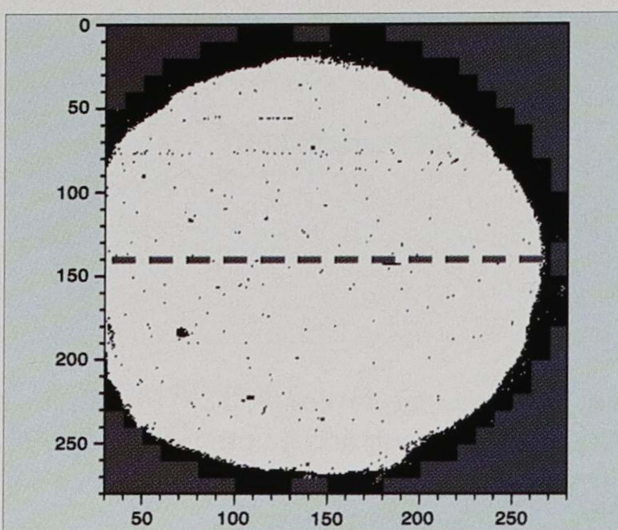
Fig. 4. Wafer map of a 3 inch bottom-emitting VCSEL wafer. The dark dots are VCSELs out of specification, and the bright dots are good devices.
