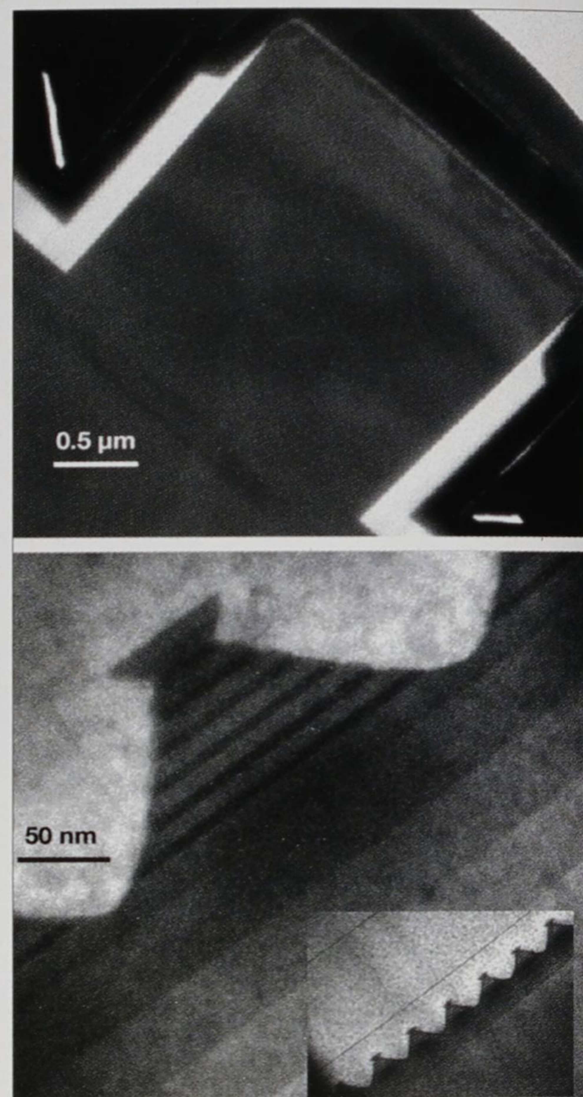
Fig. 6. TEM images of the same DFB laser. The top image is taken perpendicular to the ridge, while the lower image is parallel to the ridge, and shows details of the InGaAsP quantum wells and laser grating (inset).
