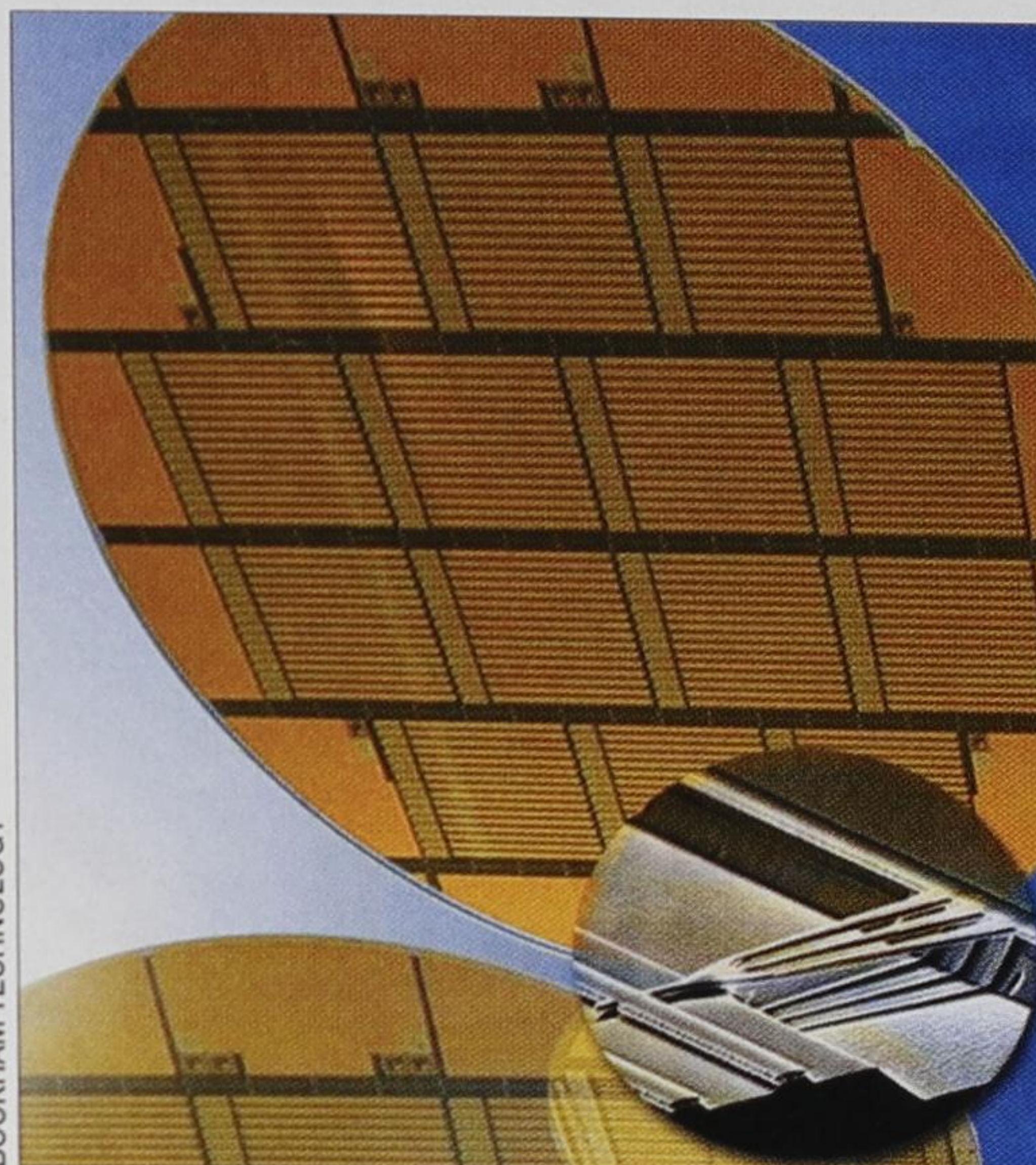
A processed 6 inch GaAs wafer showing MZ optical modulator bars. In the inset SEM image, two waveguide arms can be seen as ridges. The air bridge contacting the right ridge feeds the RF signal to the modulator arm.
