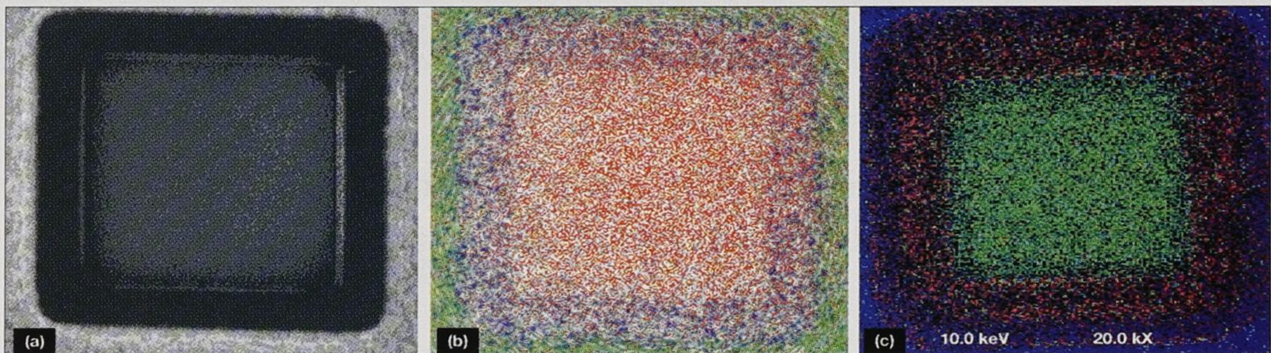
Fig. 2. (a) SEM and (b) EDX images of a 2 \mu m contact hole in an HBT device. In the EDX image the green contrast is Au, the blue is Si and the red corresponds to Ga. (c) AES image of the same HBT providing additional information on the Pd surface metal (the blue contrast represents Pd, the red indicates Si and the green indicates Ga).
