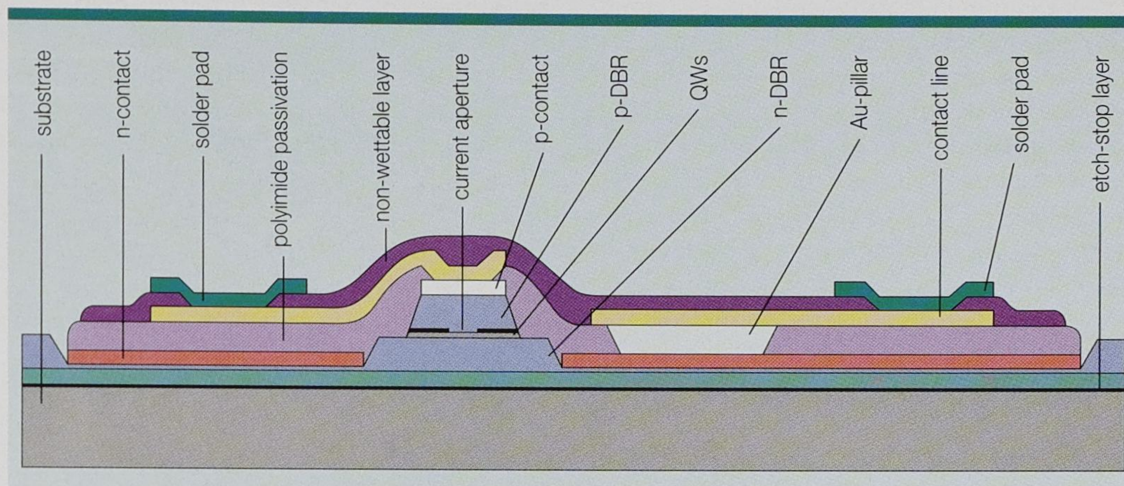
Fig. 2. Cut-away view of an ULM Photonics bottom-emitting VCSEL with solder pads for flip-chip mounting and an etch-stop layer for substrate removal.
