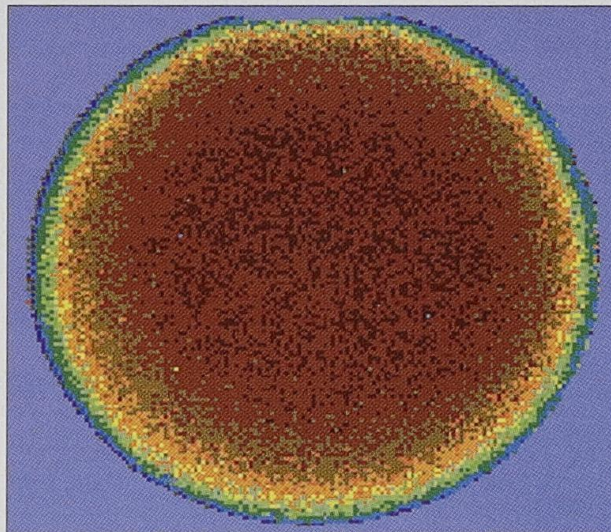
Fig. 1. PL map obtained with a resolution of 0.5 mm over a 75 mm substrate containing a 1310 nm laser epiwafer structure. A full spectrum was acquired at each position and the entire map was completed in 3 minutes.
