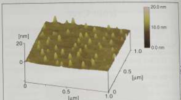
AFM image of a 3-layer stack of \text{In}_{0.2}\text{Ga}_{0.8}\text{N} quantum dots embedded in 5 \text{ nm} \text{In}_{0.02}\text{Ga}_{0.98}\text{N} spacer layers. The average diameter and width of the QDs is 19.5 \text{ nm} and 4.5 \text{ nm} , respectively.
