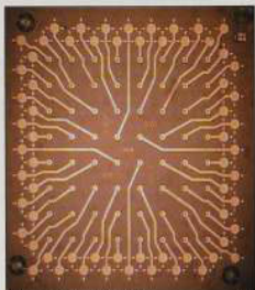
Figure 3. 8 x 8 VCSEL array measuring 2.8 mm 2 for integration into optical interconnects. The array is bonded to an intermediate sapphire substrate and subsequently to a PCB. Each VCSEL is capable of 1 Gb/s data rates and is individually addressable, allowing operation speeds of up to 64 Gb/s.
