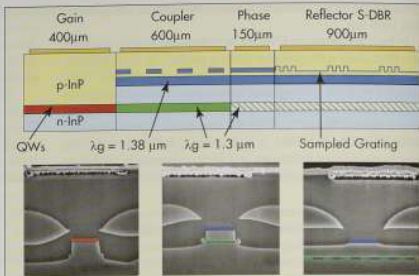
Figure 3. Cross-section of Altitun's grating coupler sampled reflector laser. The three images show profiles through the gain, coupler and reflector (and phase) sections. The output wavelength is controlled by four separate currents, one for each of the sections.
