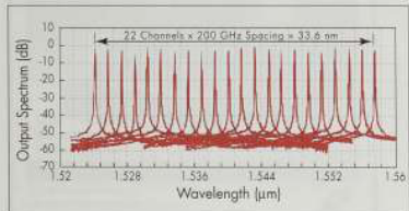
Figure 2. Spectrum of a tunable DFB laser array. The channel separation is 200 GHz, resulting in 22 channels within a 33.6 nm tuning window.
