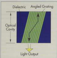
Top view of an angled-grating ( \alpha -DFB) laser.
