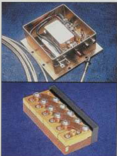
Top: FAP diode lasers are available in the 650-690 nm wavelength regime. Bottom: water-cooled linear array CW bars in 50 and 60 W versions operate in the range 780-840 nm.
