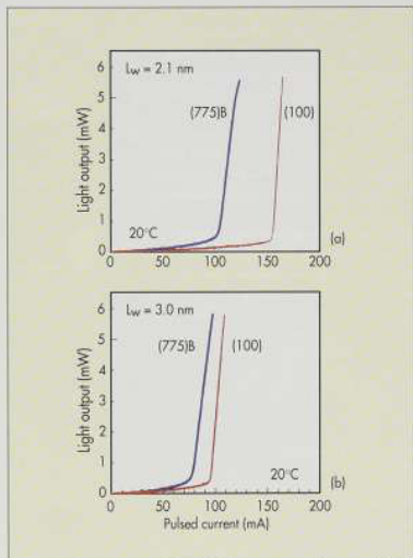
Fig. 2. I-L curves for the (775)B quantum wire- and (100) GRIN-SCH lasers with: a) well width ( L_w ) = 2.1 nm and b) L_w = 3.0 nm.
