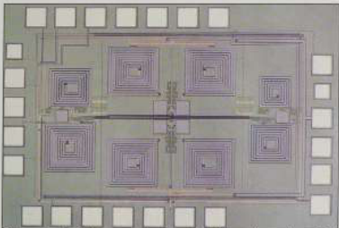
Photograph of the transmitter die, which has dimensions 1.3 x 0.85 mm 2 . Each inductor (the purple-colored spirals) is integrated without further processing steps and consists of a stack of three structures made of three metal layers. This reduces the area by around a factor of eight.
