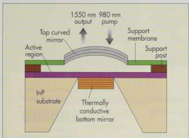
Figure 4. CoreTek's tunable VCSEL has a micromachined top mirror which is displaced by an electrostatic force, varying the cavity length and the output wavelength.
