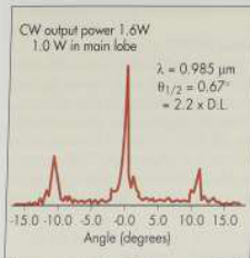
Figure 4. CW far-field pattern of a 40-element, near-resonant antiresonant array. When operated at 9x threshold current, the output power is 1.6 W CW with 1.0 W in the main lobe. The wallplug efficiency is 23% [16].
