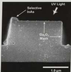
Figure 7. This GaAs mesa was exposed to UV light from the direction of the top right hand corner, forming a modified oxide mask on the exposed facets. InAs was grown selectively on the unexposed left-hand facet.
