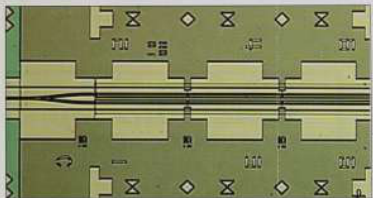
Figure 1. Top view of Nortel's tunable DFB array. Three grating sections on each of two waveguides provide a 33.6 nm tuning range. The waveguides are combined to provide a single output, at left.
