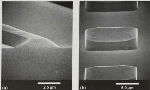
Figure 2. Selective InAs growth on resistlessly patterned GaAs wafers. (a) shows a line along the [010] direction, while (b) shows squares with a vertical facet for orientation along [011].
