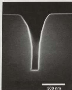
Figure 3. Sub-300 nm spacing between selectively grown InAs lines.
