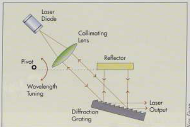
Figure 5. A Littman-Metcalf external cavity diode laser. The cavity is formed between the rear facet of a Fabry-Perot laser diode and an adjustable, external reflector.
