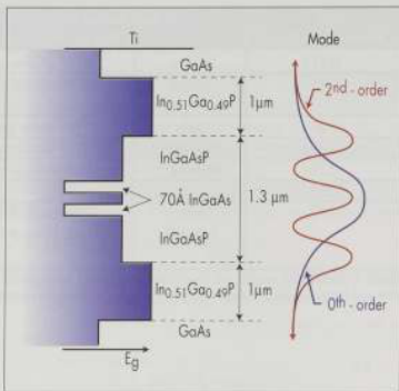
Figure 2. Schematic representation of an Al-free, broad-waveguide 0.97 \mu\text{m} -emitting diode laser [5]. Devices with this structure recently demonstrated record-high CW and quasi-CW powers of 16.8W and 23.5W respectively, from 200 \mu\text{m} -stripe devices [6].
