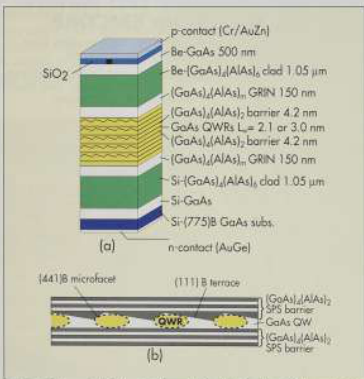
Fig. 1. Schematic illustration of the GaAs(GaAs) 4 (AlAs) 2 GRIN-SCH quantum wire (QWR) laser structure grown on (775)B GaAs substrates by MBE: a) entire laser structure and b) quantum wire region.
