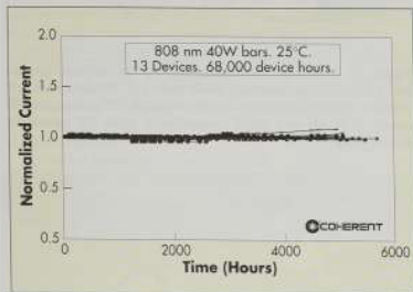
Figure 3. Lifetests at 40 W CW for 1 cm laser bars emitting at 0.81 \mu\text{m} . These ALFA-type devices, manufactured by Coherent, contain a single tensile-strained InGaAsP quantum well with Al-free waveguiding layers and AlInGaP cladding layers [10].
