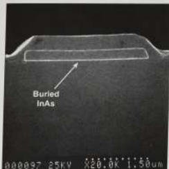
Figure 6. Following selective growth of InAs (rectangular shape, center), the oxide mask was removed in-situ allowing regrowth of GaAs to form an embedded structure.
