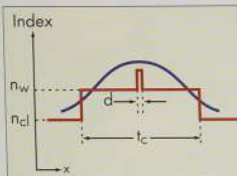
Figure 1. Schematic representation of a broad waveguide (BW) laser structure, showing the effective-index profile (red) and the field-intensity profile (blue).
