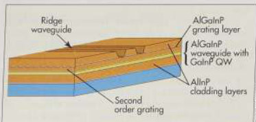
Schematic of SDL's 662 nm DFB laser, which provides 90 mW CW output power.
