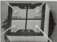
Figure 2. An SEM microphotograph of the 2 x 2 VCSEL array (seen in figure 1). The VCSELs are spaced at 125 µm intervals and have an aperture size of 5 µm. The device dimension is 0.75 x 0.75 mm².
