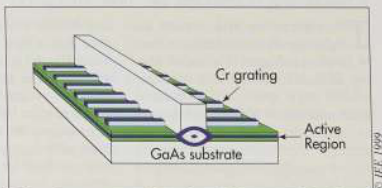
Schematic structure of the electrically pumped ZnSe-based DFB laser. The active region contains a CdZnSe SQW between ZnSse waveguides.
