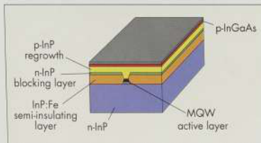
Schematic cross-section of a semi-insulating planar buried heterostructure (SIPBH) laser with an Fe-doped InP semi-insulating layer.
