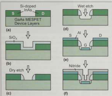
Figure 4. Process schematic for resistless MESFET fabrication. (a) Selective deposition of n-InAs source and drain contact regions, (b) \text{SiO}_x deposition, (c) anisotropic dry etch, (d) wet etch, (e) metallization, (f) nitride deposition.
