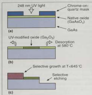
Figure 1. Schematic of the resistless patterning process. (a) The native oxide on GaAs is modified selectively by exposure to UV light through a mask. (b) The unexposed native oxide is desorbed, leaving a surface patterned with UV-modified oxide. (c) The UV-modified oxide acts as a mask for selective etching or growth (below the desorption temperature of Ga 2 O 3 ).
