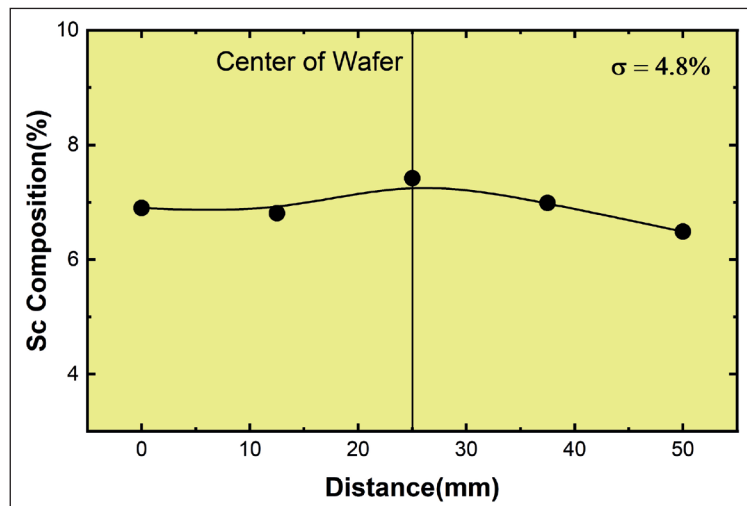
➤ Figure 7. Composition of a ScAlN film measured by Rutherford backscattering spectroscopy across the diameter of a 50 mm wafer. The average composition and coefficient of variation are 7 percent and 4.8 percent, respectively.
