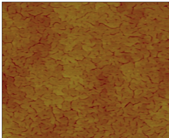
➤ Figure 8. A 2 \mu\text{m} by 2 \mu\text{m} scan of a ScAlN/GaN HEMT structure grown on SiC. The root-mean-square (RMS) roughness is 0.20 nm.
