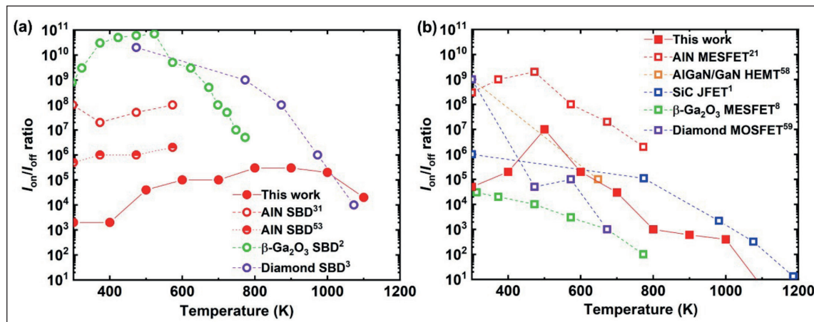
➤ Figure 6. A benchmarking plot, comparing the current on-off ratio versus measurement temperature of AlN devices with the other state-of-art (a) Schottky barrier diodes and (b) FETs.
