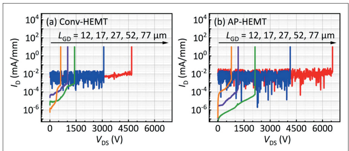
► Figure 4. The off-state characteristics of the conventional GaN HEMT (a) are inferior to the variant with the active-passivation design (b).
