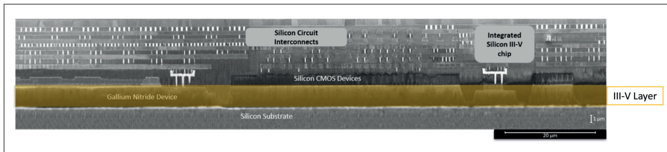
► Figure 4: A transmission electron microscopy cross-section of a finished 200 mm wafer processed using silicon foundry manufacturing. The tungsten plug process used for the BEOL is used to also connect to the III-V FEOL.
