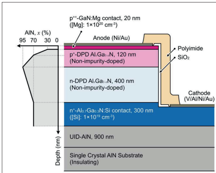
➤ Figure 7. Distributed polarisation doping is used to form the AlN-based diode.
