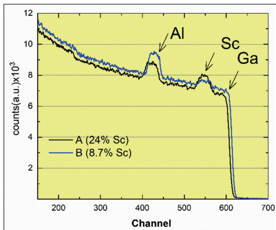
➤ Figure 5. Rutherford backscattering spectroscopy of ScAlN alloys grown on GaN-on-sapphire templates using Agnitron's Agilis 100. The blue trace shows around 9 percent scandium, while the black trace shows 24 percent.
