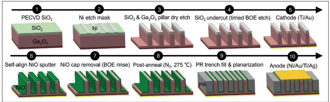
➤ Figure 6. The ten-step process to produce \text{Ga}_2\text{O}_3 superjunction Schottky barrier diodes.
