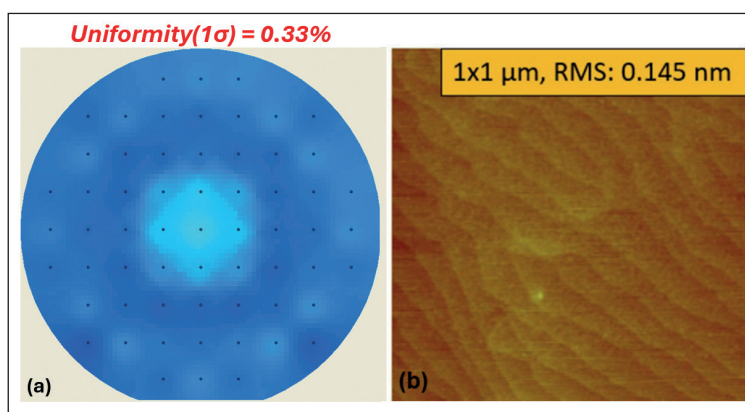
➤ Figure 4. (a) Thickness map for a 0.73 \mu\text{m} -thick AlN film and (b) an atomic force microscopy image of a 2 \mu\text{m} -thick AlN layer on a sapphire substrate. Notably, these films showcase exceptional smoothness, with a uniformity of less than 0.33 percent.
