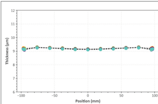
On-Wafer thickness uniformity: (Max-Min)/mean = \pm 0.8 - 1.0\%
