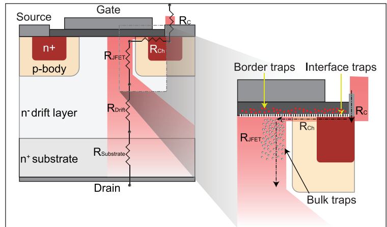
➤ Figure 1. An illustration of a vertical power MOSFET. The inset shows the region where the current transport occurs from the source to the drain. Also shown is the location of the border, the interface, and the bulk traps generated as a consequence of thermal oxidation.
