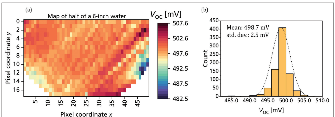
► Figure 3. (a) Open-circuit voltage ( V_{oc} ) map of a 6-inch InP-on-GaAs substrate populated with InGaAs laser power converters. Each pixel with coordinate ( x,y ) corresponds to an individual device with a nominal area of 5.4 \text{ mm}^2 . A total of 826 cells were processed and measured. The photocurrent density was on average 7.98 \text{ A cm}^{-2} with a standard deviation of 0.11 \text{ A cm}^{-2} . The V_{oc} performances are reported in histograms in (b).
