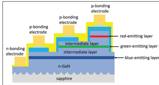
➤ Toyoda Gosei's full-colour monolithic microLED.
