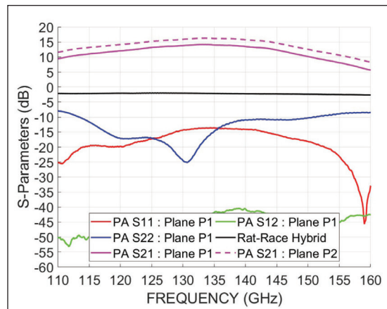
➤ Figure 6. Solid lines represent the small signal S-parameters of the PA at reference plane P1. By subtracting the loss of the rat-race hybrid (black line) from the S21 of the PA between P1-P1 (solid magenta), the reference plane can be shifted to the S21 of the PA between P2-P2 (dashed magenta).
