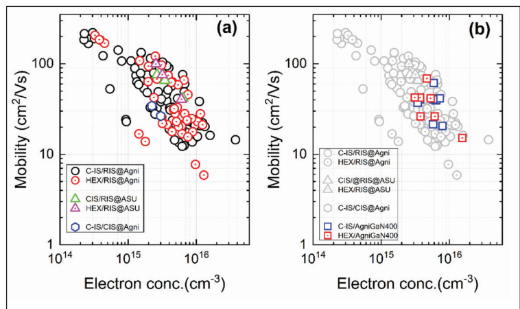
► Figure 2. Electron mobility as a function of free-electron concentration in intentionally silicon-doped AlN layers grown by MOCVD under varying growth conditions. (a) Results from Agilis 100 reactors: remote-injection showerhead (RIS) at Agnitron (circles), close-injection showerhead (CIS) at Agnitron (hexagons), and RIS at Arizona State University (triangles). (b) Results from AlN layers grown using the AgniGaN 400 horizontal reactor (squares), compared with data from the Agilis reactors. Different colours indicate the substrate used for growth.
