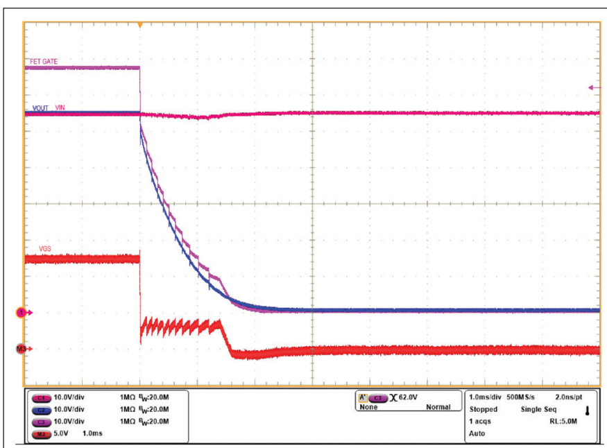
➤ Figure 5. Short-circuit response of the LM50661 controller with eight MOSFETs.
