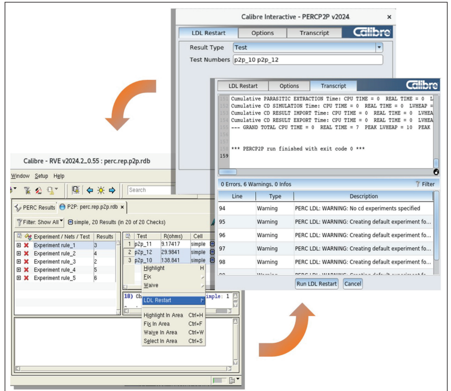
➤ Figure 3. Run Calibre PERC P2P Debug simulations on select P2P results directly from the debug GUI.
