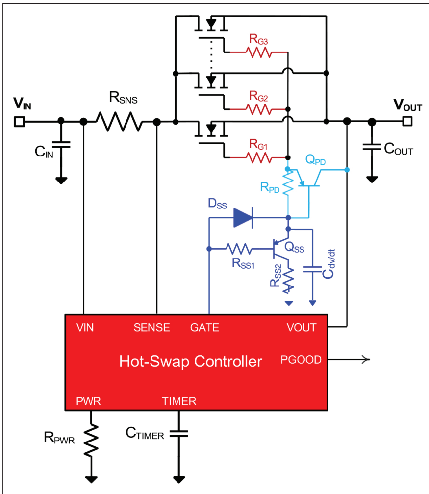
➤ Figure 8. Proposed hot-swap circuit configuration.
