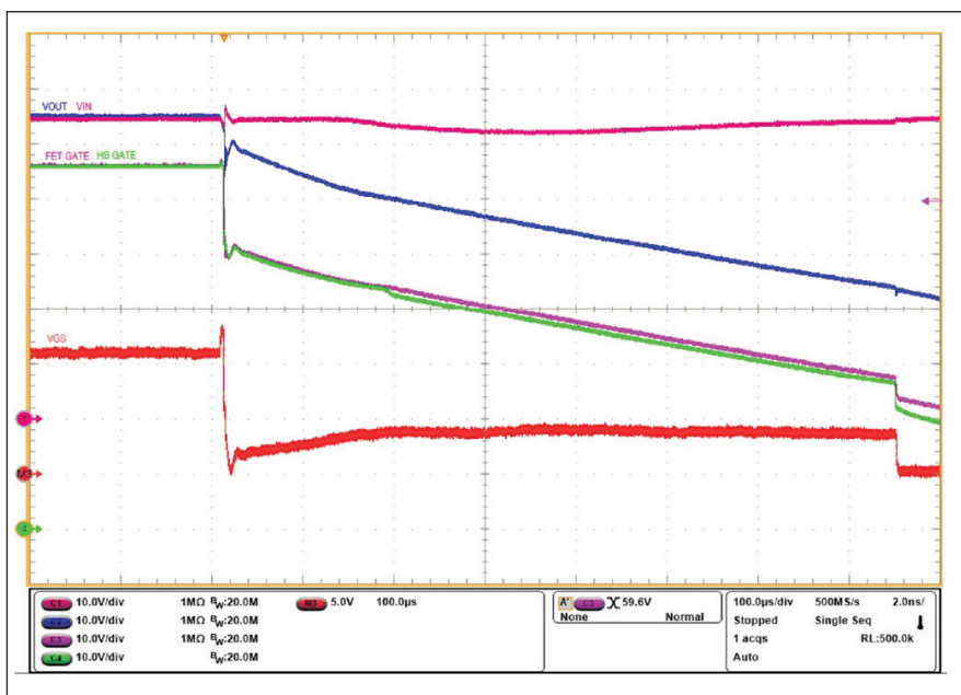
➤ Figure 9. Output short-circuit response with fast pull-down circuit.
