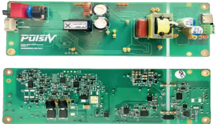
► Below: Pulsiv PS V-E BAD65USB Evaluation Board.
