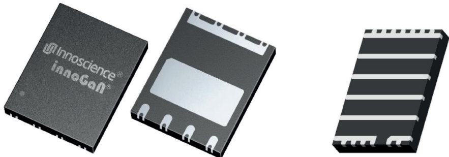
► Far Left Duo: Innoscience INN700DA240B and right: Innoscience INN150FQ032A.
