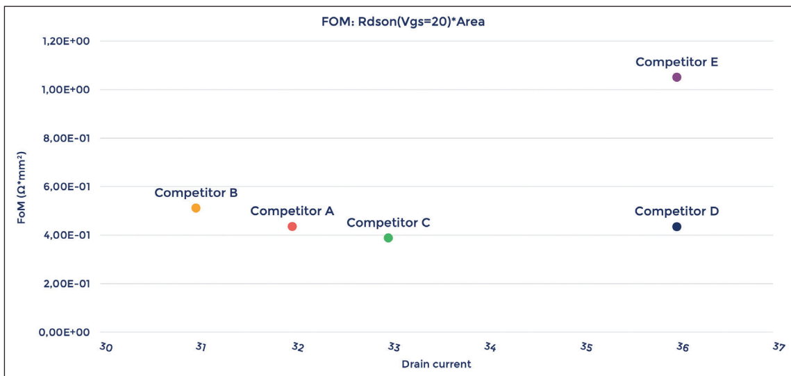
► Performance comparison of discrete SiC MOSFETs figure of merit.
