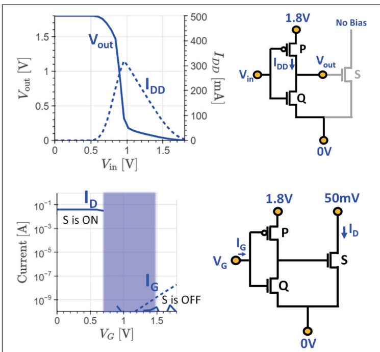
➤ Figure 10. (Top) Transfer characteristics, V_{\text{out}} - V_{\text{in}} , of the GaN-silicon CMOS driver, P and Q, in DrGaN technology. (Bottom) The steady-state transfer characteristics of DrGaN. The switching of the GaN power switch, S, is driven by the integrated GaN-silicon CMOS driver (P and Q). Turning on involves a driver pull-up to a V G rail of 1.8 V, and turning off involves a driver pull-down to a V G rail of 0 V.
