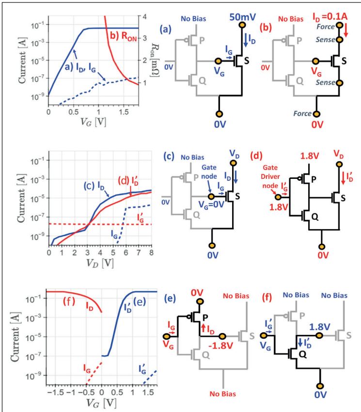
➤ Figure 9. (Top) the transfer characteristics of the GaN power switch S with a total width of 421.1 mm in DrGaN, demonstrating transistor operation. The normalized R_{\text{DSON}} is 0.8 mΩ mm 2 . (Middle) The leakage characteristics, I_b - I_b - V_D and I_b' - I_b' - V_D of the GaN power switch S in DrGaN, in the off-state accomplished by either applying a bias voltage, V_G , of (c) 0 V directly at the gate node of S; or (d) 1.8 V at the gate driver node of P and Q. (Bottom) The I-V transfer characteristics of the (e) silicon PMOS, P, and (f) GaN NMOS, Q, in the gate driver of DrGaN.
