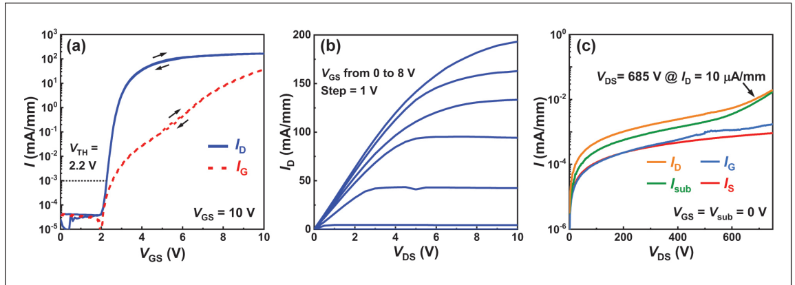
► Figure 5. (a) Transfer and gate leakage, (b) output and (c) off-state leakage characteristics of the E-mode p -GaN gate HEMT on the same platform with the BiPFET.
