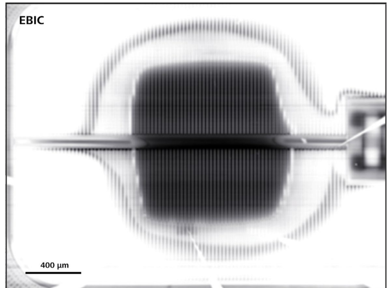
➤ Figure 4: Low magnification EBIC analysis showing signals from the entire width of the chip. The analysis is taken from the location on one of the metallized emitter lines, as shown in the lower center.
