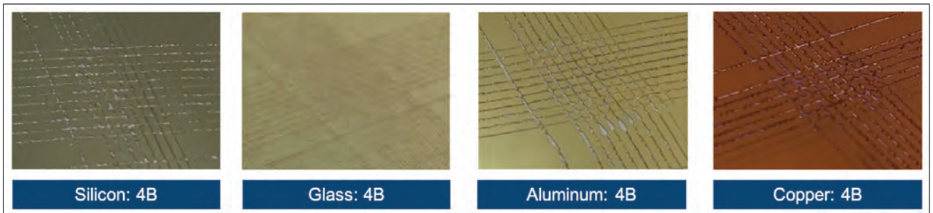
► Figure 3. Cross hatch tape peel testing suggests good adhesion of low-loss PID material to various substrates, including Si, Glass, Al, and Ti/Cu surfaces
